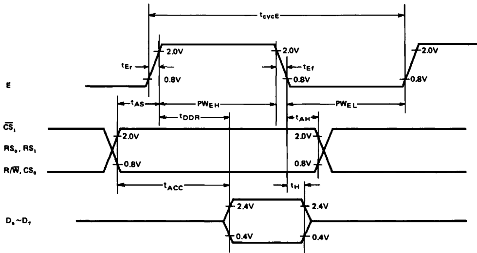
Figure 5 Read Timing
