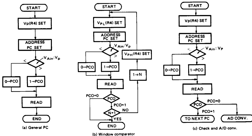
Figure 20 PC Application Flow Chart Examples
