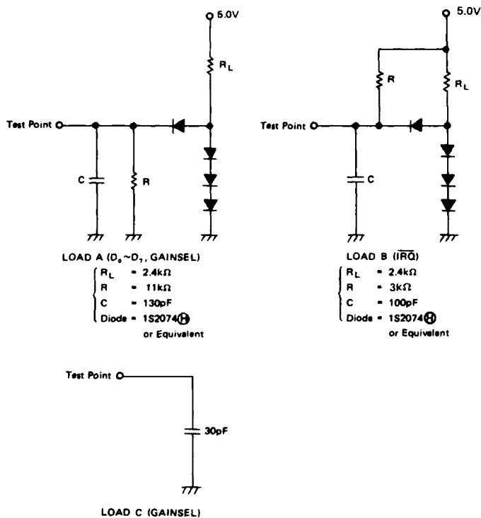
Figure 7 Test Load
