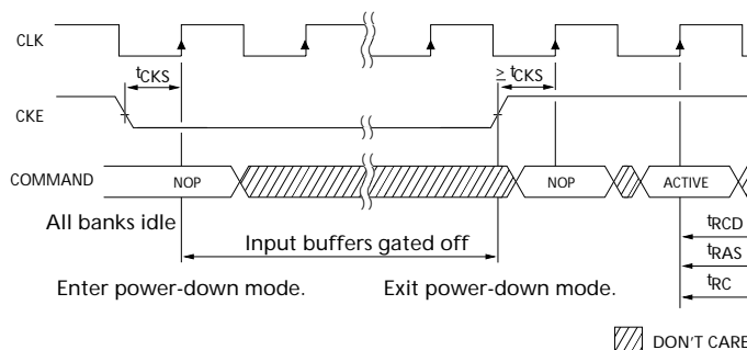
Figure 21 Power-Down
