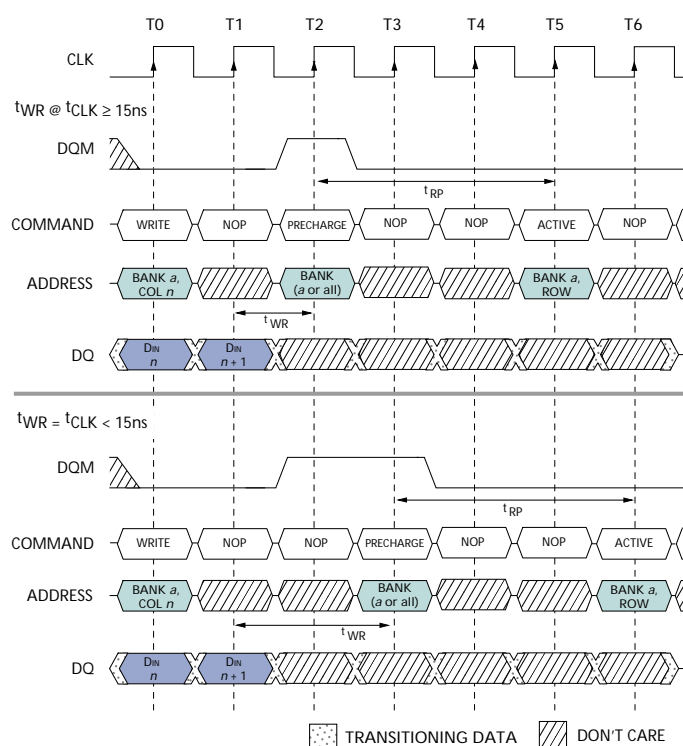
Figure 18 WRITE To PRECHARGE
