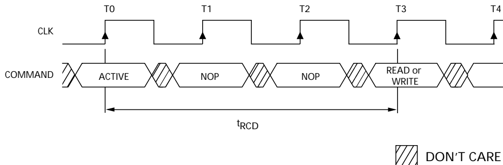
Figure 4 Example: Meeting t_{RCD}(\text{MIN}) When 2 < t_{RCD}(\text{MIN})/t_{CK} \leq 3
