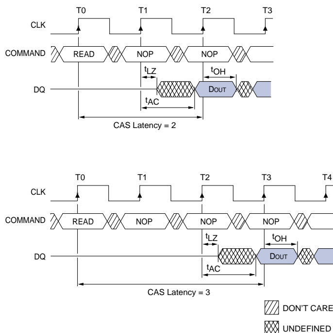
Figure 6 CAS Latency
