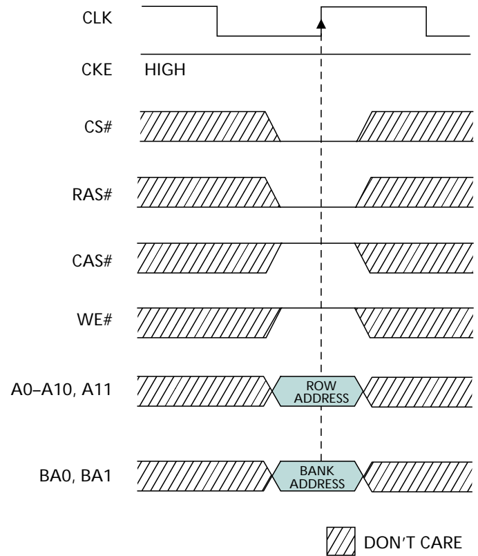
Figure 4 Example: Meeting t_{RCD}(\text{MIN}) When 2 < t_{RCD}(\text{MIN})/t_{CK} \leq 3
