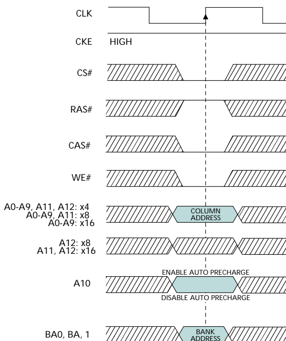
Figure 13 WRITE Command
