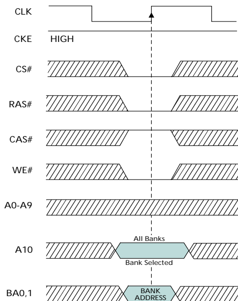
Figure 20 PRECHARGE Command
