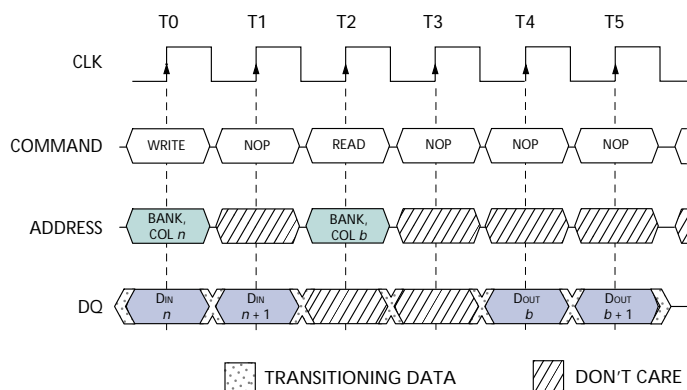
Figure 17 WRITE To READ
