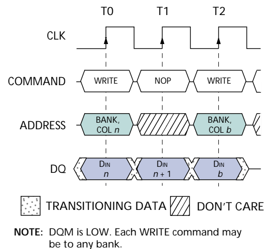
Figure 15 WRITE to WRITE
