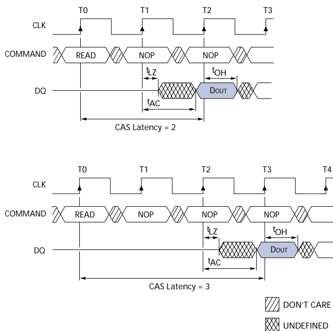
Figure 2 CAS Latency
