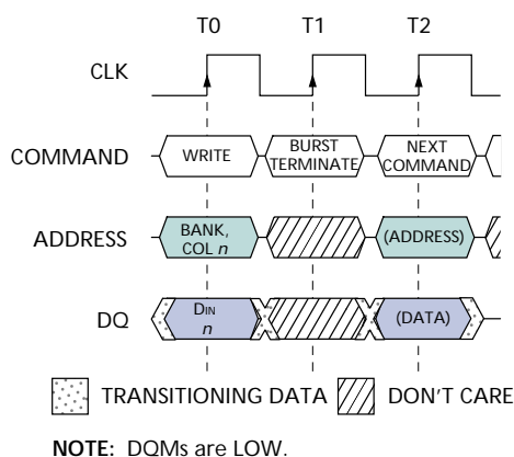
Figure 19 Terminating a WRITE Burst
