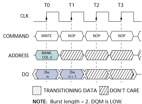
Figure 14 WRITE Burst
