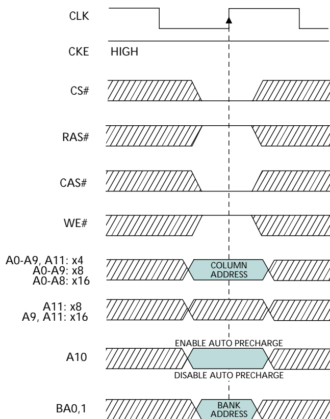
Figure 5 READ Command
