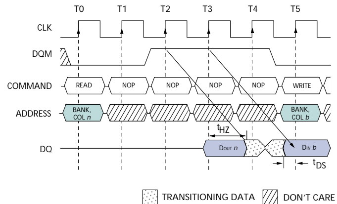
Figure 10 READ to WRITE with Extra Clock Cycle
