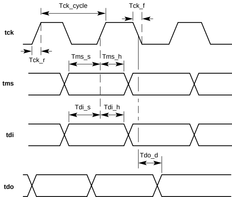
Figure 20 JTAG Boundary-Scan Timing Diagram
