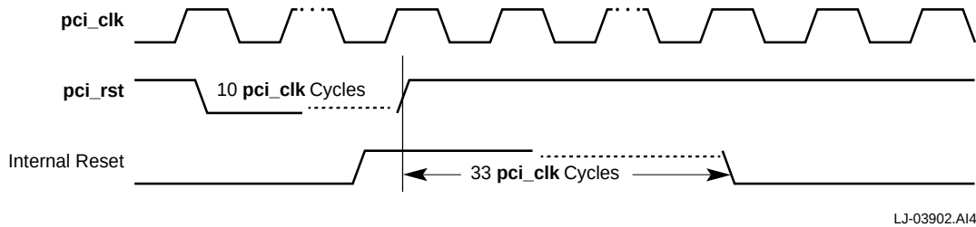
Figure 3 PCI Reset Timing Diagram
