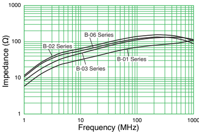
Impedance Characteristics
