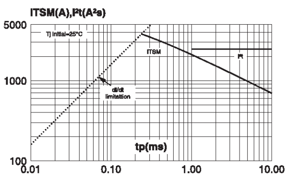
Fig. 6-2: Non repetitive surge peak on-state current for a sinusoidal pulse with width t_p < 10 ms, and corresponding value of I t (MDS80).
