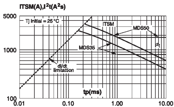
Fig. 6-1: Non-repetitive surge peak on-state current for a sinusoidal pulse with width t_p < 10 ms, and corresponding value of I t (MDS35 and MDS50).
