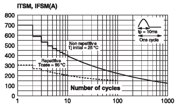
Fig. 6-2: Non repetitive surge peak on-state current for a sinusoidal pulse with width t_p < 10 ms, and corresponding value of I t (MDS80).
