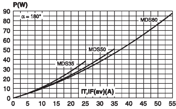
Fig. 1-3: Maximum total power dissipation versus output current on resistive or inductive load (Single phase bridge rectifier, two packages).
