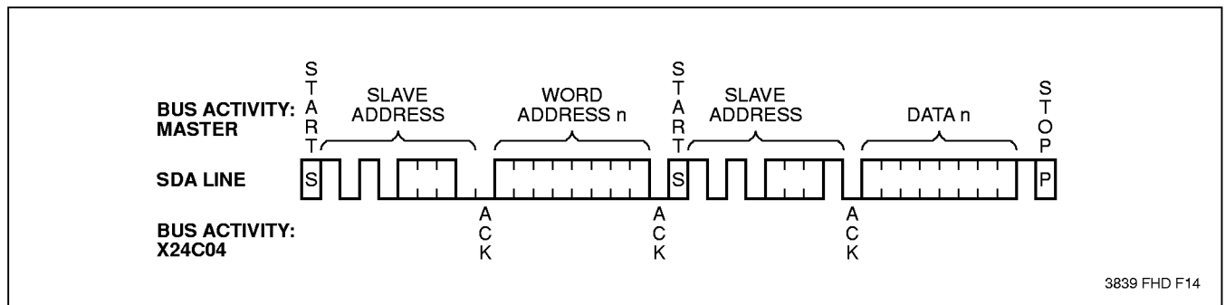
Figure 8. Random Read
