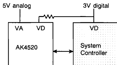
Case 3. 5V/3V system
