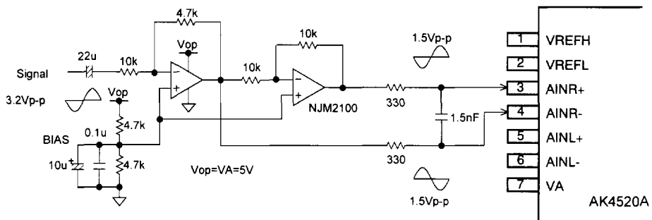
Figure 9. Differential Input Buffer Example
