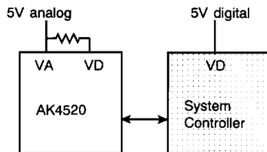
Case 1. 5V system
