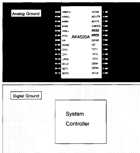
Figure 7. Ground Layout
