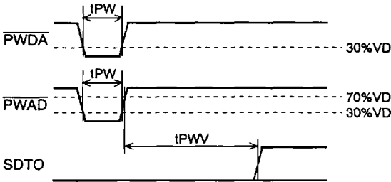
Reset & Initialize Timing
