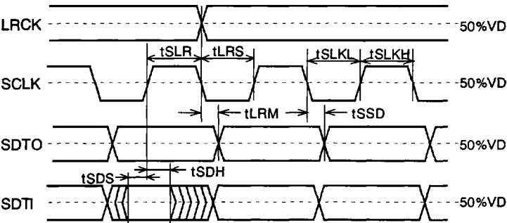
Serial Interface Timing
