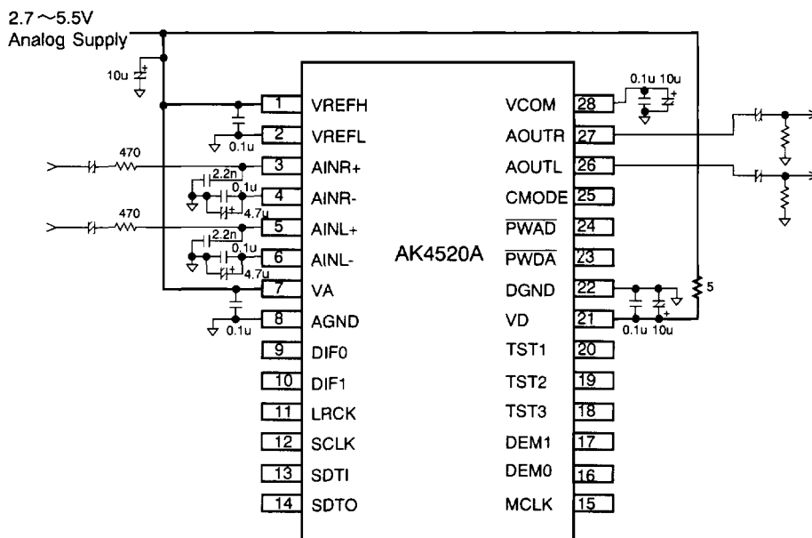
Figure 6. Typical Connection Diagram
