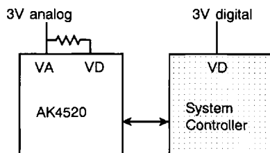
Case 2. 3V system
