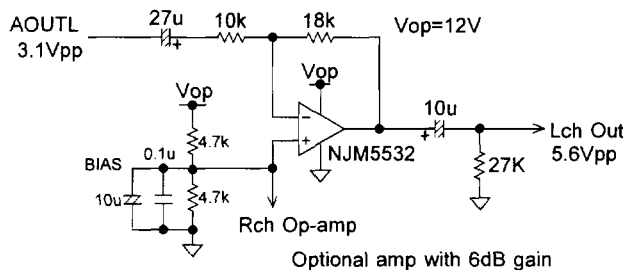
Figure 10. External analog circuit example(gain=6dB)
