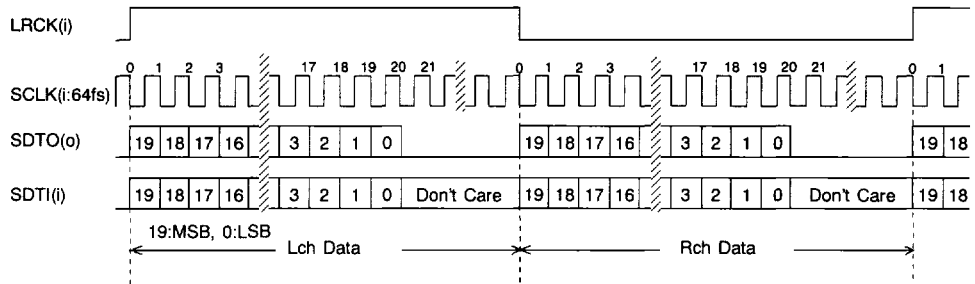
Figure 3. Mode 2 Timing
