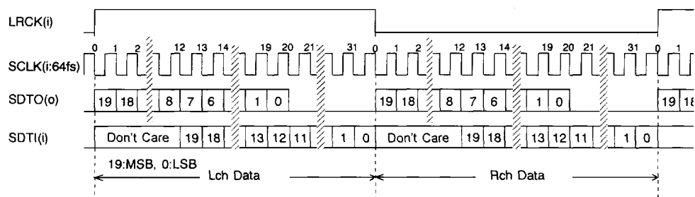
Figure 2. Mode 1 Timing
