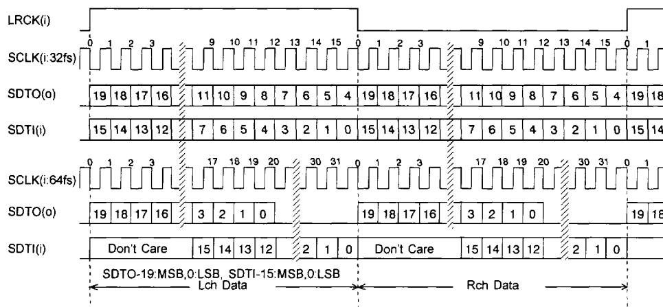
Figure 1. Mode 0 Timing
