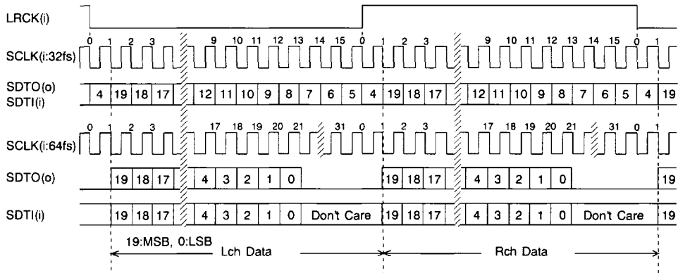
Figure 4. Mode 3 Timing
