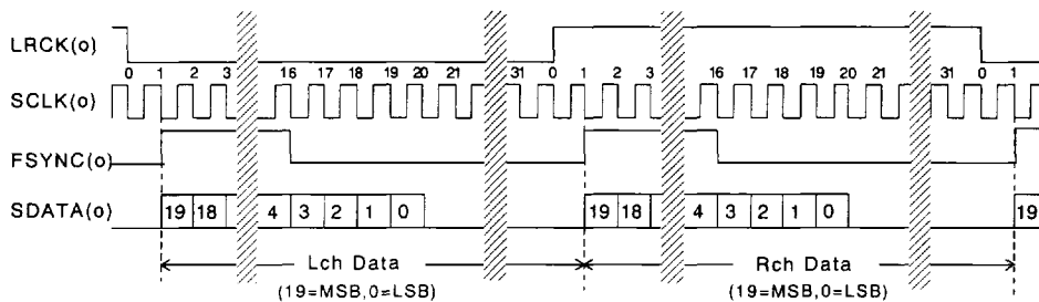
Figure 4. Data Output Timing (I 2 S Master mode)
