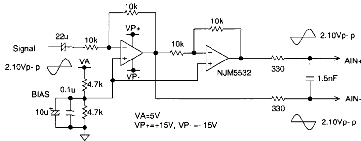
Figure 6. Full-differential Input Buffer Circuit Example
