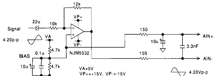
Figure 7. Single-ended Input Buffer Circuit Example
