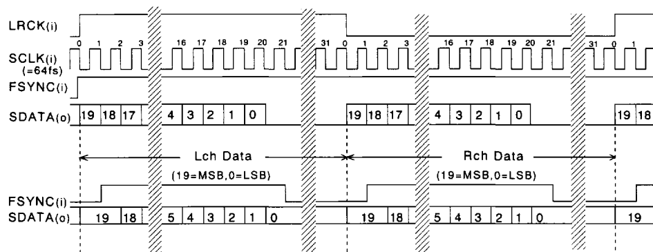
Figure 1. Data Output Timing (Slave mode)
