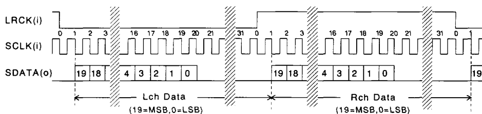
Figure 3. Data Output Timing(I 2 S Slave mode)
