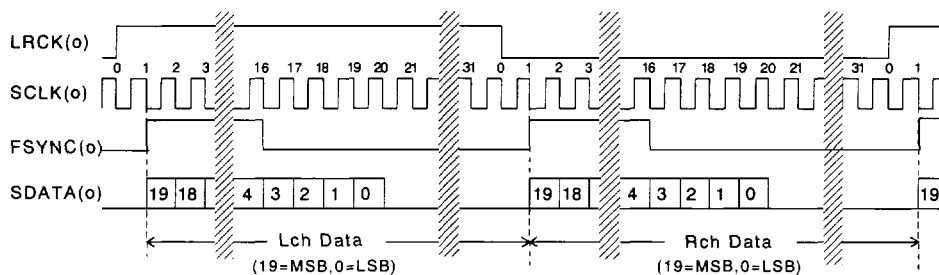
Figure 2. Data Output Timing(Master mode)
