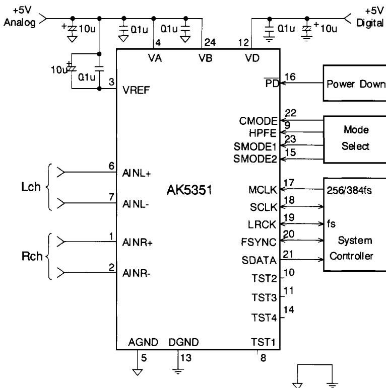
Figure 5. System Connection Diagram Example
