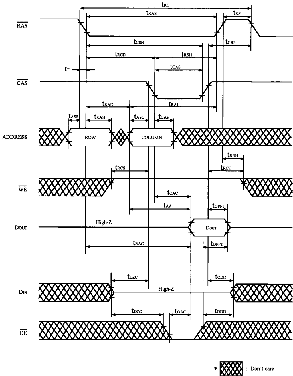
FIGURE 1. READ CYCLE
