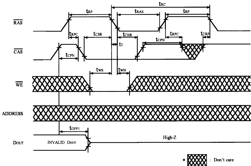
FIGURE 12. TEST MODE CYCLE
