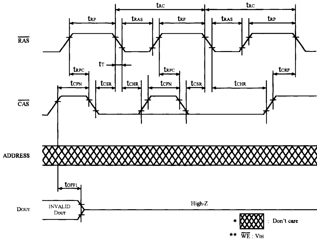
FIGURE 6. \overline{\text{CAS}} BEFORE \overline{\text{RAS}} REFRESH CYCLE
