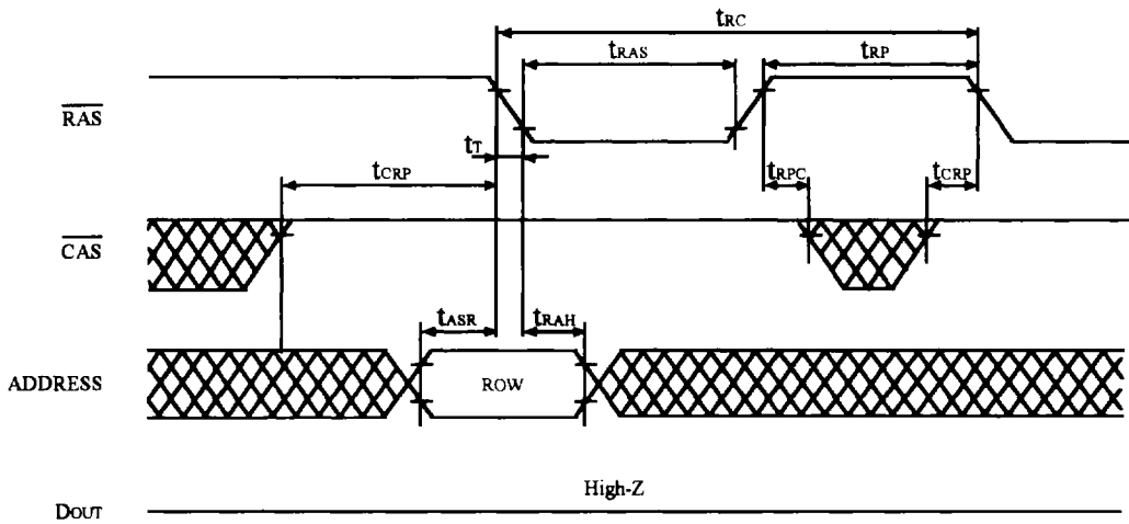
FIGURE 5. \overline{\text{RAS}} ONLY REFRESH CYCLE
