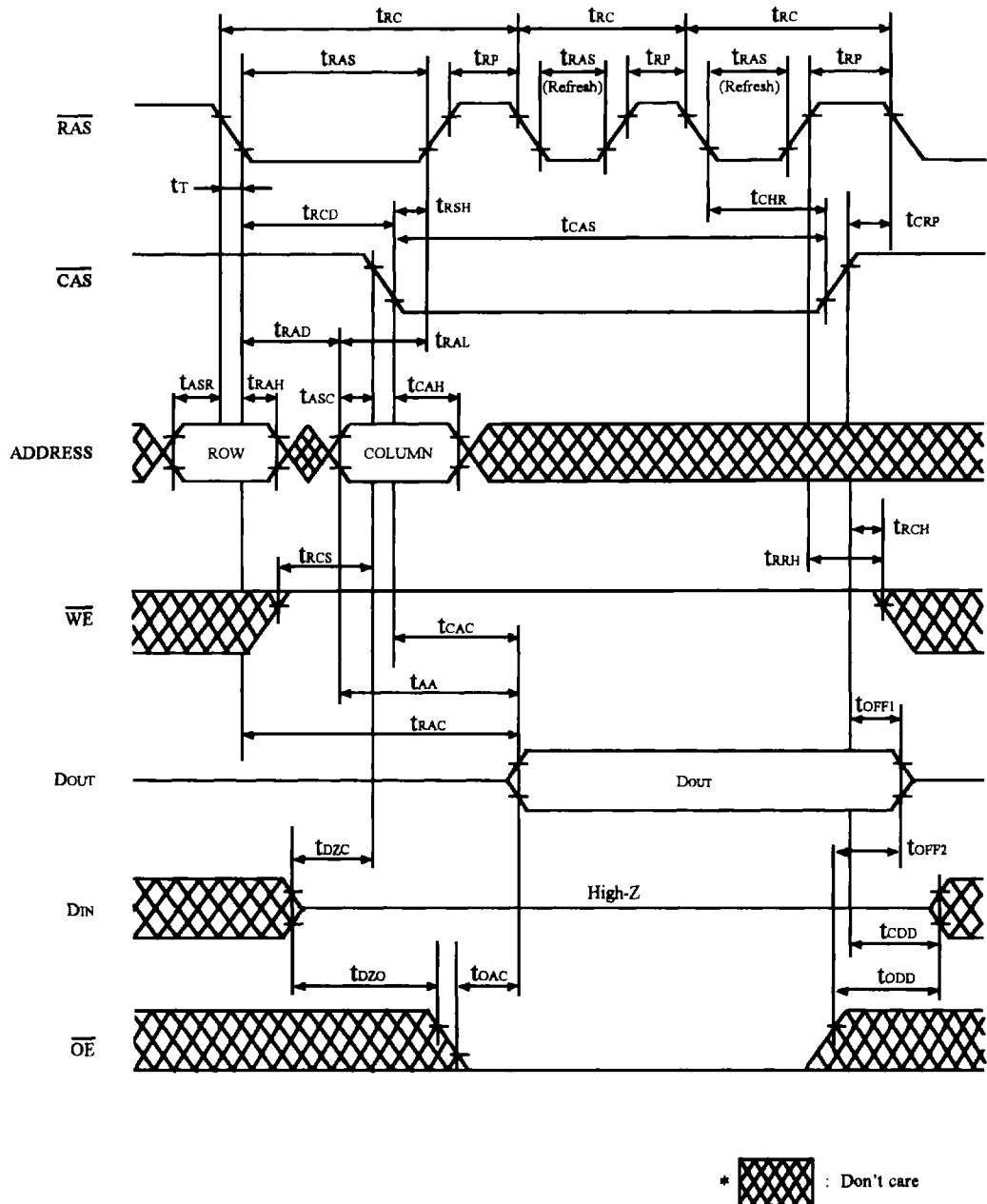
FIGURE 7. HIDDEN REFRESH CYCLE
