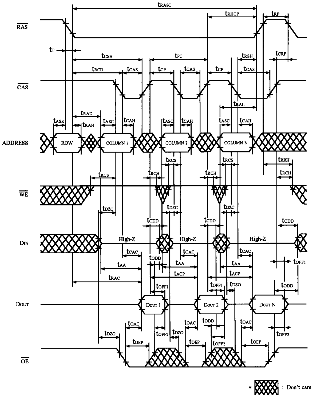
FIGURE 8. FAST PAGE MODE READ CYCLE
