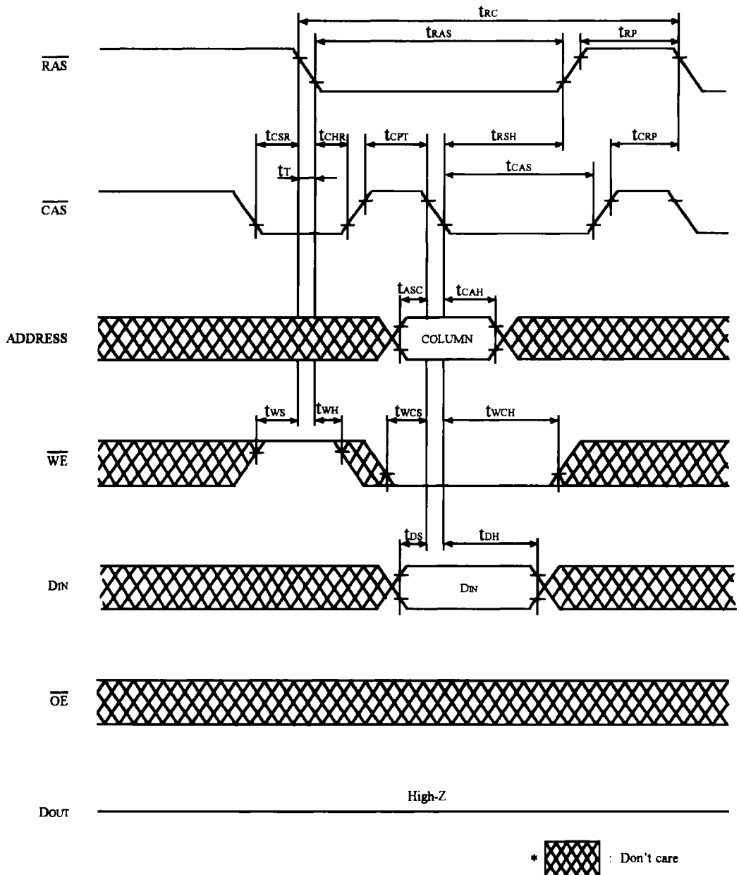
FIGURE 17. \overline{\text{CAS}} BEFORE \overline{\text{RAS}} REFRESH COUNTER CHECK CYCLE (WRITE)
