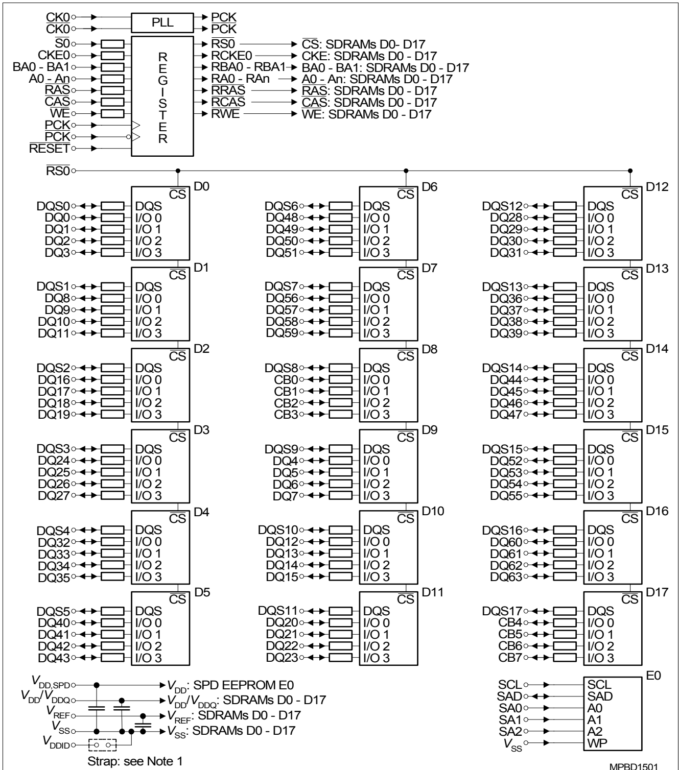
Figure 3 Block Diagram Raw Card C x72 1 Rank x4, ECC
