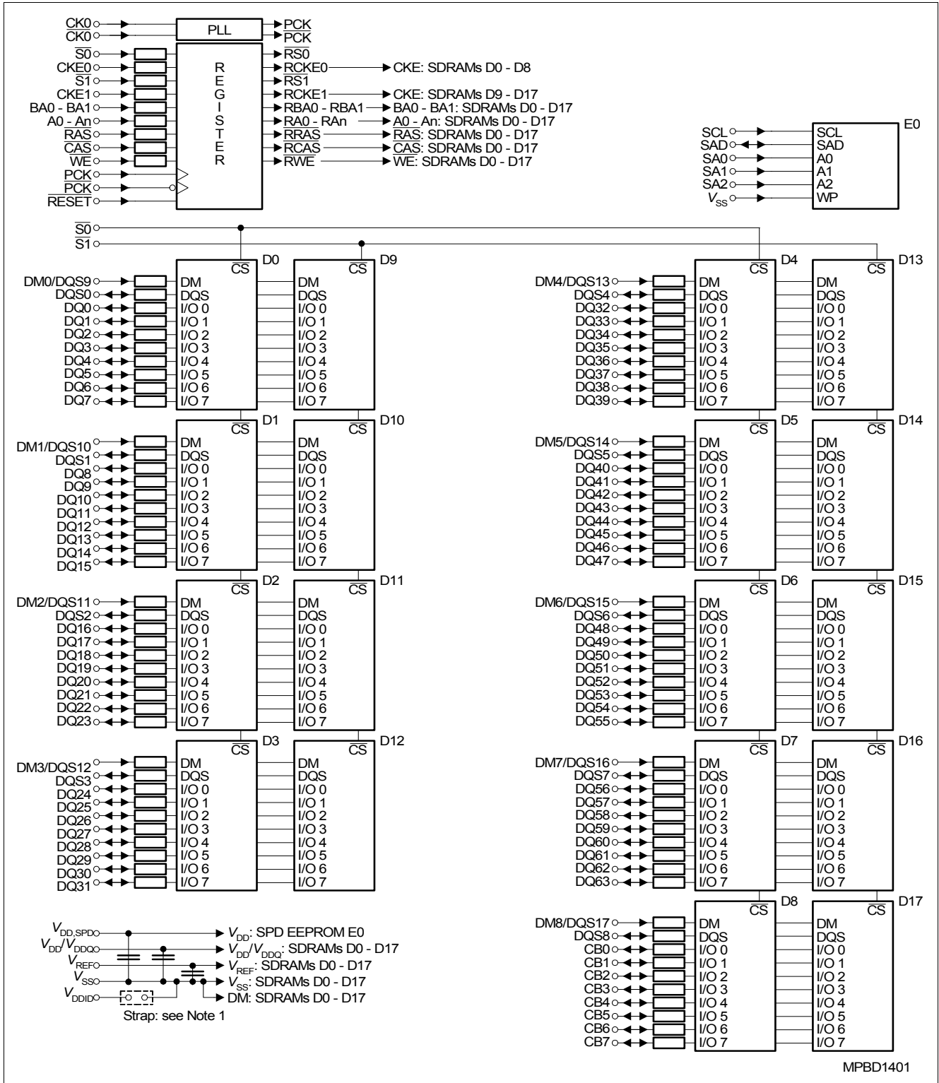
Figure 4 Block Diagram Raw Card B x72, 2Ranks x8, ECC
