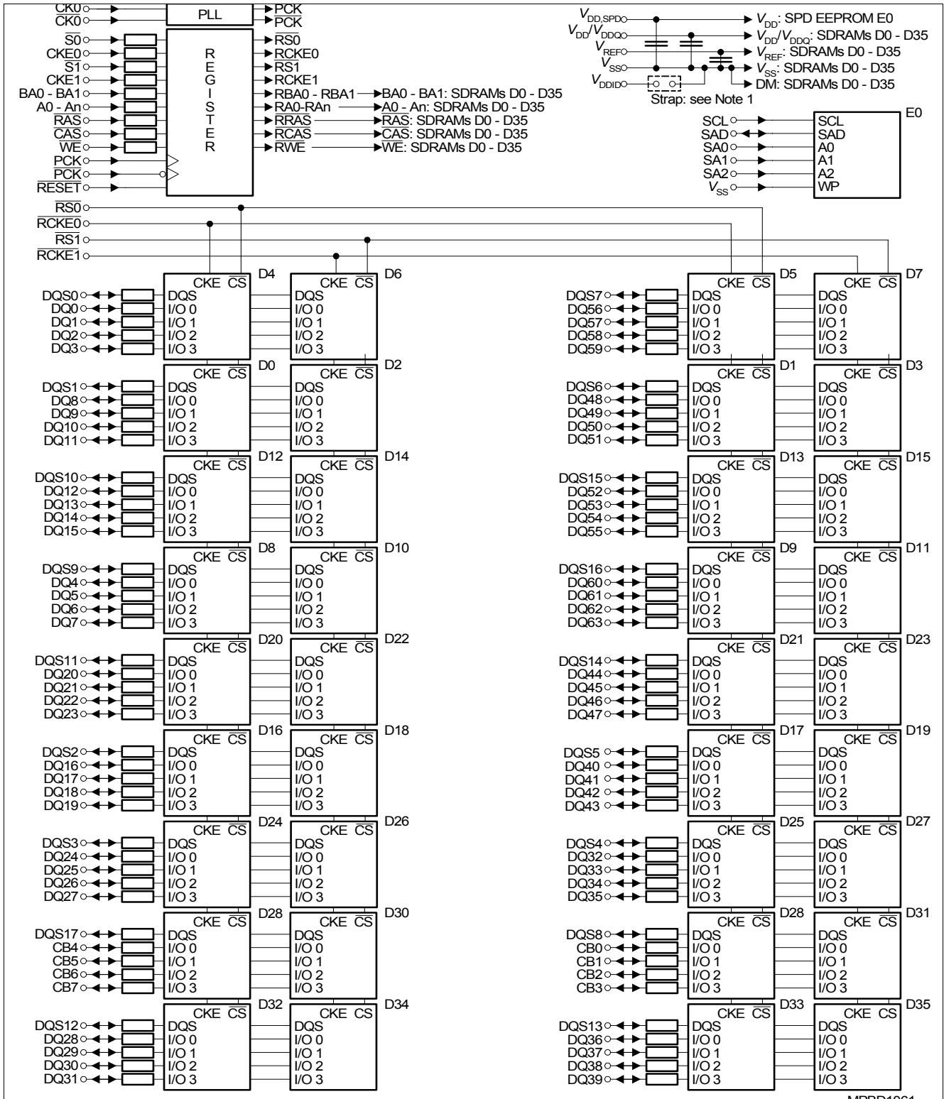
Figure 6 Block Diagram Raw Card D / F x72 2 Ranks x4, ECC
