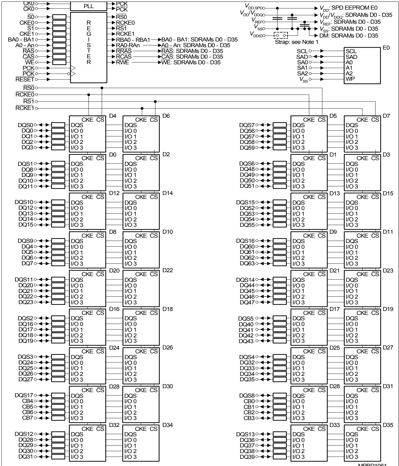
Figure 5 Block Diagram Raw Card D / F x72 2 Ranks x4, ECC
