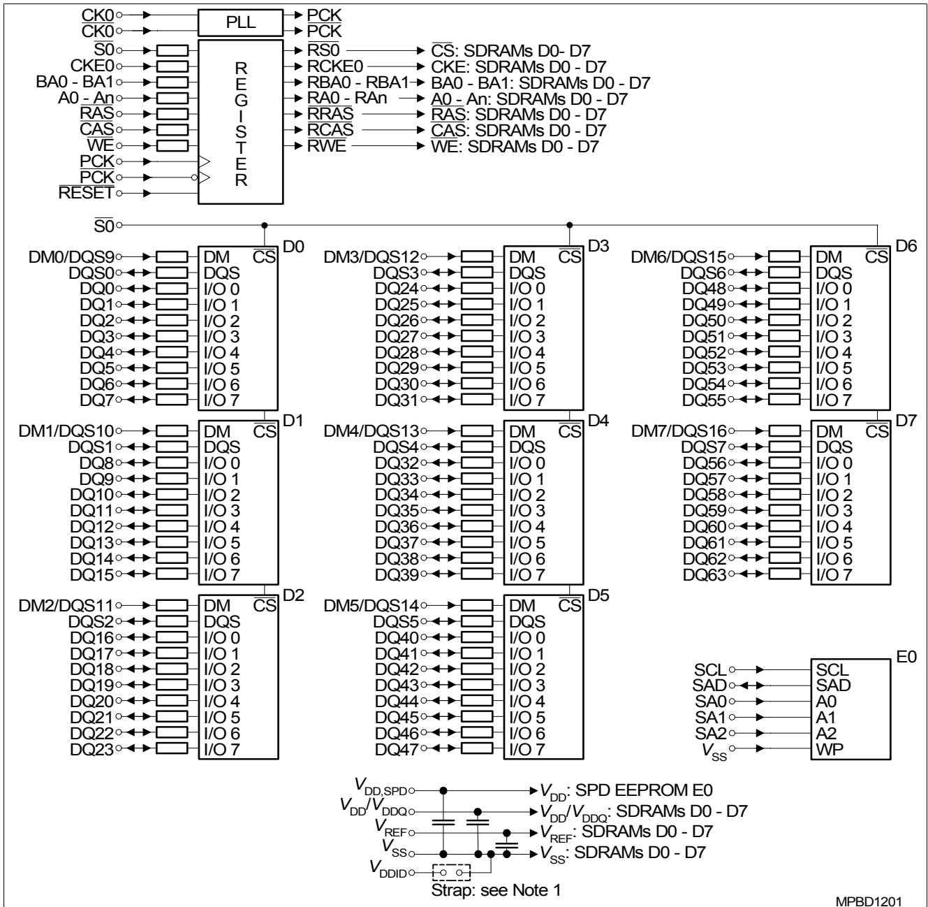
Figure 2 Block Diagram RDIMM Raw Card A x64, 1Rank, x8
