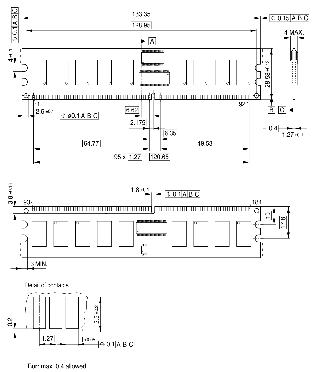
Figure 7 Package Outline Raw Card C – L-DIM-184-22-2
