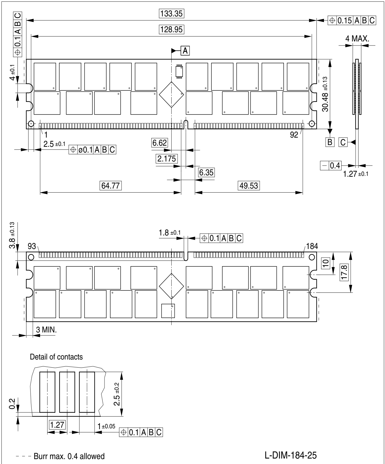
Figure 9 Package Outline Raw Card D – L-DIM-184-25
