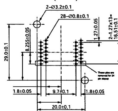
SOP IC51-0282-986 (28 Pins)
