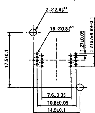
SOP IC51-0162-658 (16 Pins)
