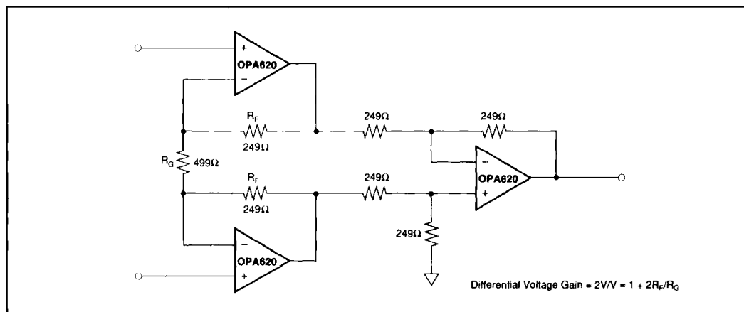
FIGURE 15. Wideband, Fast-Settling Instrumentation Amplifier.
