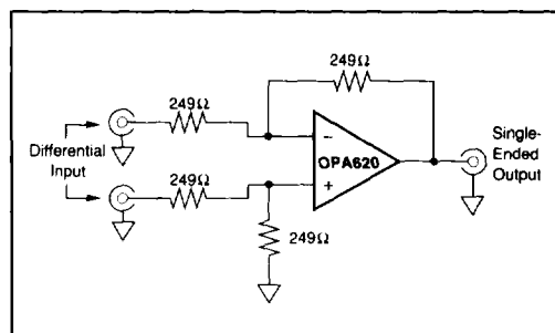
FIGURE 16. Unity Gain Difference Amplifier.
