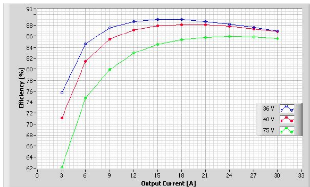
Figure 2. Efficiency vs. load current and input voltage for SQE48T30010 converter mounted horizontally. Convection cooled with T_a = 25 °C.
