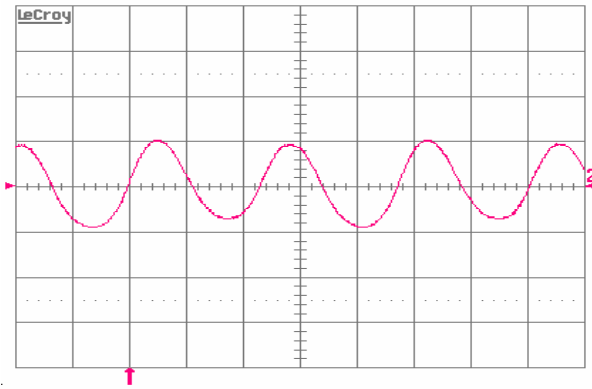
Figure 13. Input reflected ripple-current, i_c (100 mA/div.), measured at input terminals at full rated load current and V_{in} = 48 V. Refer to Fig. 12 for test setup. Time scale: 1 \mu s/div.
