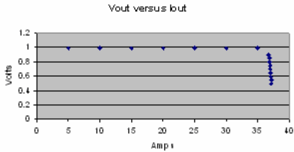
Figure 14. Output voltage vs. load current showing current limit point and converter shutdown point. Input voltage has almost no effect on current limit characteristic.
