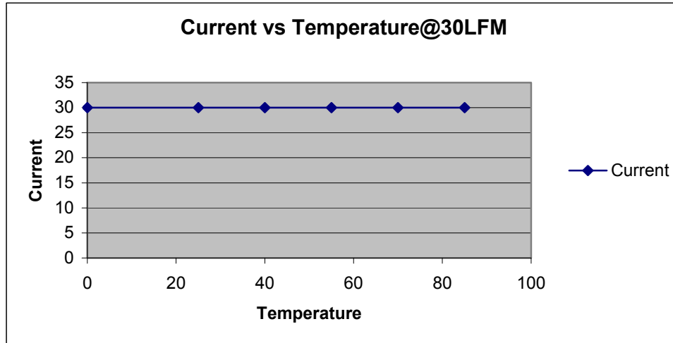
Figure 1. Available load current vs. ambient air temperature for an SQE48T30010 converter mounted vertically with air flowing from pin 3 to pin 1, MOSFET temperature \leq 125 °C, V_{in} = 48 V.
