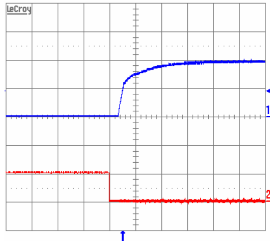
Figure 7. Turn-on transient at full rated load current (resistive) plus 10,000 \mu F at Vin = 48 V, 30 Amps and turned on using ON/OFF pin. Top trace, Iout=Output voltage (0.5 V/div.). Bottom trace: ON/OFF signal (5 V/div.). Time scale: 2 ms/div.
