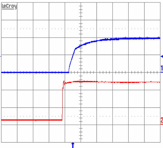
Figure 5. Vin versus output voltage for SQE48T30010 converter mounted horizontally. Vin=48Vdc, Iout= 30 Amps, Cout=10,000uF and turned on using Vcc. Convection cooled with Ta=25°C. Top trace: Output voltage (0.5 V/div.). Bottom trace: VCC (20 V/div.). Time scale: 2 ms/div. Convection cooled with Ta=25°C.
