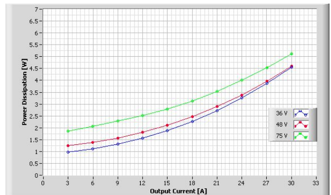
Figure 3. Power dissipation vs. load current and for SQE48T30010 converter mounted horizontally. Convection cooled with T_a = 25 °C.
