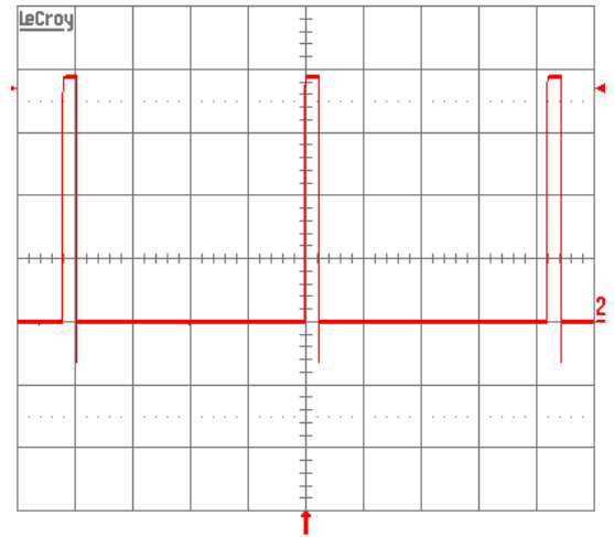
Figure 15. Load current (top trace, 10 A/div., 50 ms/div.) into a 10 m \Omega short circuit during restart, at V_{in} = 48 V.
