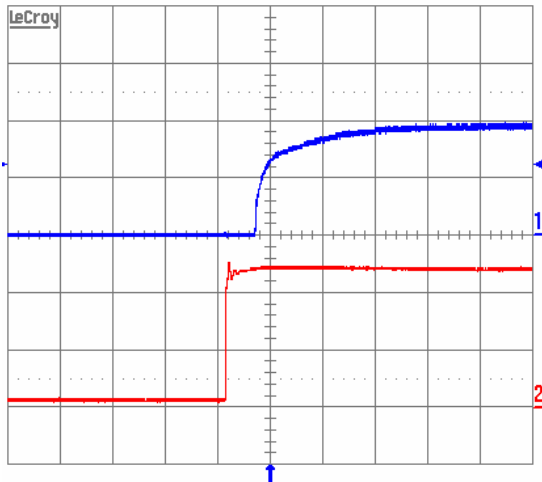
Figure 4. Vin versus output voltage for SQE48T30010 converter mounted horizontally. Vin=48Vdc, Iout=30 Amps and turned on using Vcc. Top trace: Output voltage (0.5 V/div.). Bottom trace: VCC (20 V/div.). Time scale: 2 ms/div. Convection cooled with Ta=25°C.
