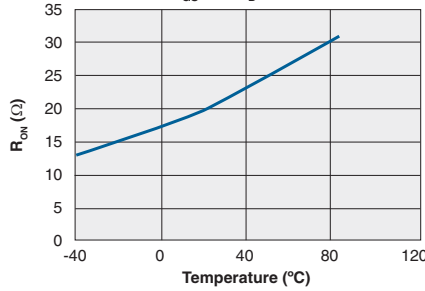
R_{ON} vs. Temperature ( V_{GS}=0\text{V}, I_D=90\text{mA} )
