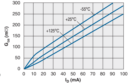
Transconductance vs. Drain Current ( V_{DS}=10\text{V} )
