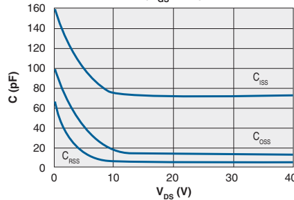
Capacitance vs. Drain Source Voltage ( V_{GS}=-5\text{V} )
