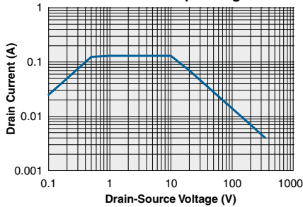
Max Rated Safe Operating Area
