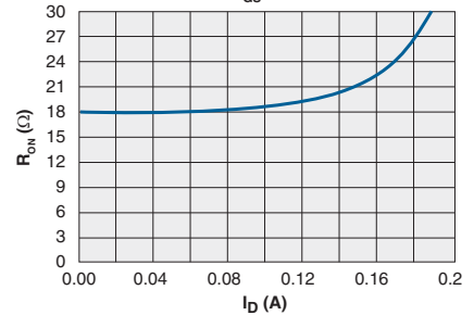
On-Resistance vs. Drain Current ( V_{GS}=0\text{V} )
