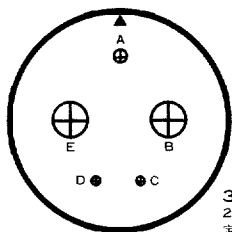
14S-5 5-#16 Serv. INST
