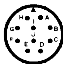
18-1 10-#16 Serv. A(BCFG) INST(Others)
