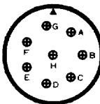
22-23 8-#12 Serv. D(H) A(Others)
