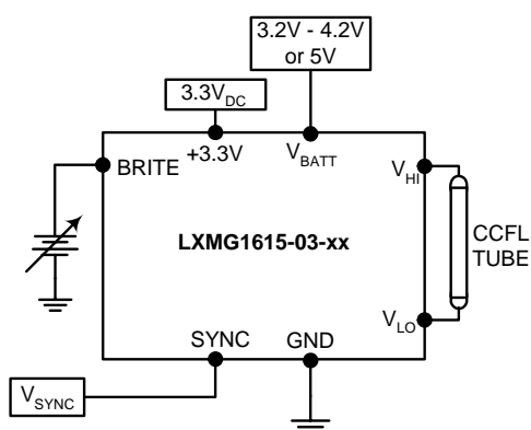
Figure 5 - Brightness Control
