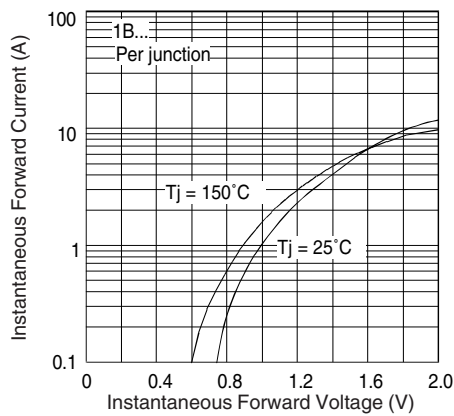
Fig. 1 - Forward Characteristics
