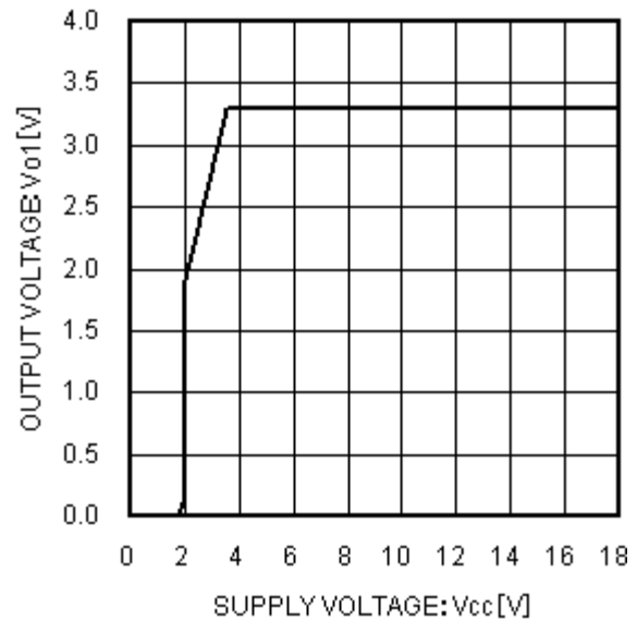
Fig.18 Input Stability (3.3 V output I_{O1}=600 mA)
