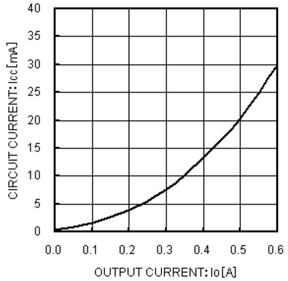
Fig.16 Circuit Current vs Load Current I_O ( I_O=0 \rightarrow 600 mA)
