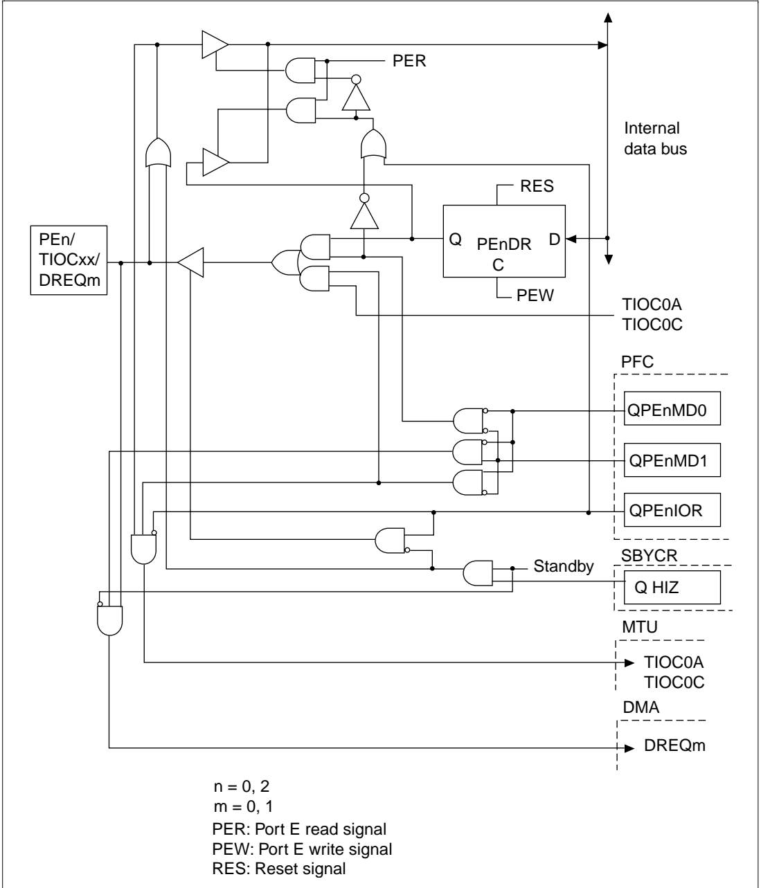
Figure B.38 PE n /TIOcXX/DREQ m Block Diagram
