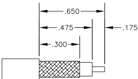
STRIPPING DIMENSIONS
