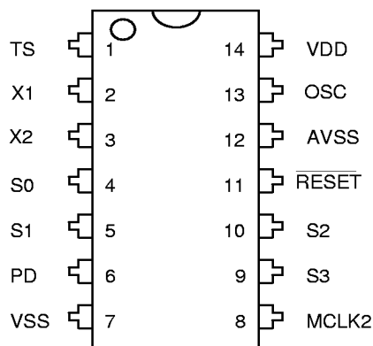
Figure 1: Connection Diagram for Plastic Dip or SOIC Package
