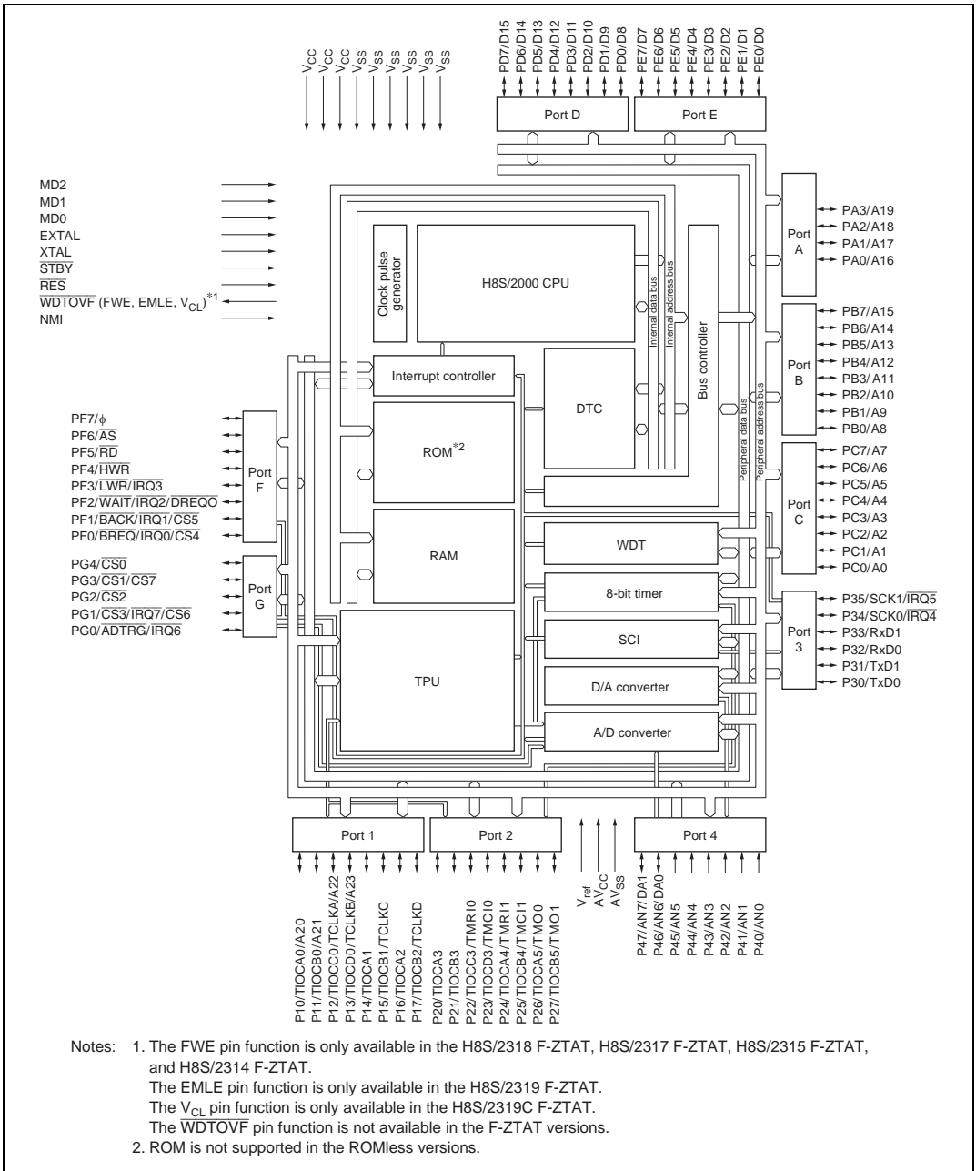
Figure 1.1 Block Diagram
