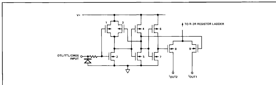
FIGURE 2: CMOS Switch
