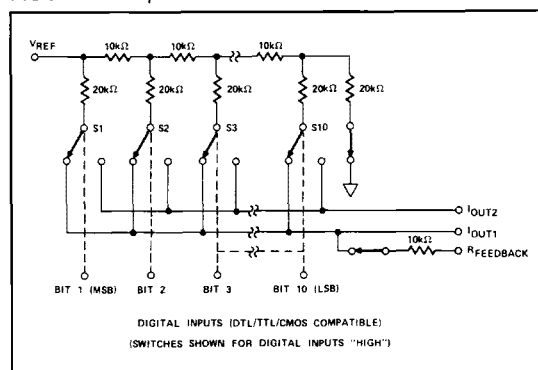
FIGURE 1: Simplified DAC Circuit
