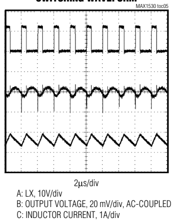
STEP-DOWN REGULATOR SWITCHING WAVEFORM
