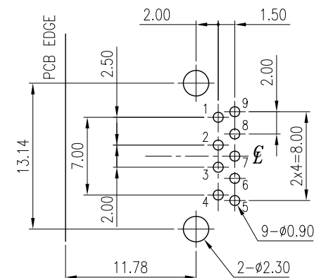
RECOMMENDED PCB LAYOUT- TOP VIEW (GENERAL TOLERANCE: ±0.05)
