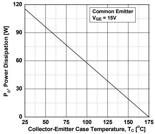
Figure 20. Power Dissipation
