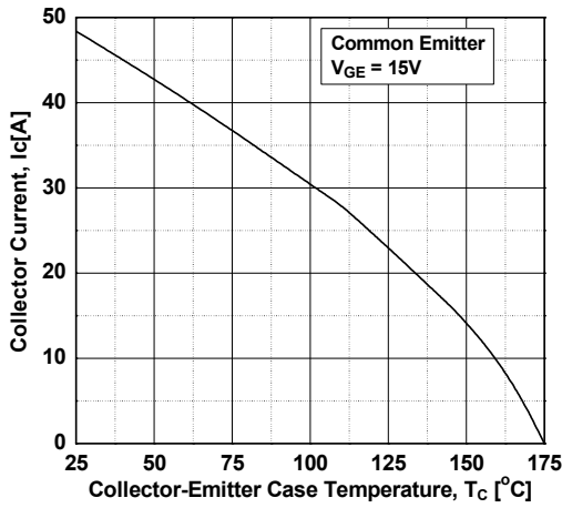
Figure 19. Current Derating
