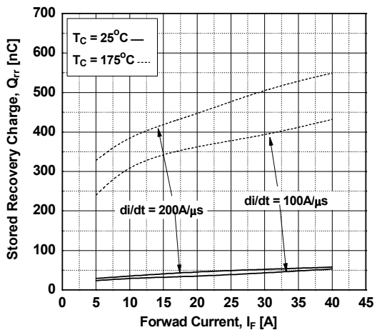
Figure 24. Stored Charge
