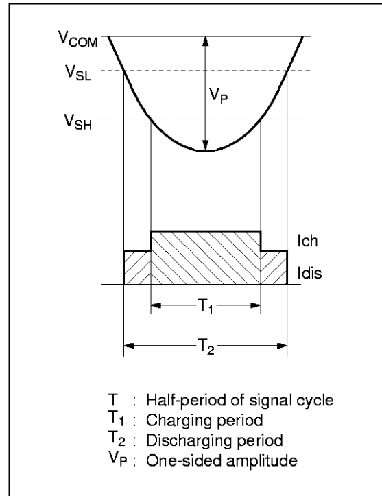
Figure 7 Charge / Discharge Timing
