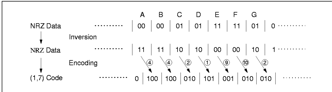
Figure 9 Shows an Example of NRZ to (1, 7) Code Conversion
