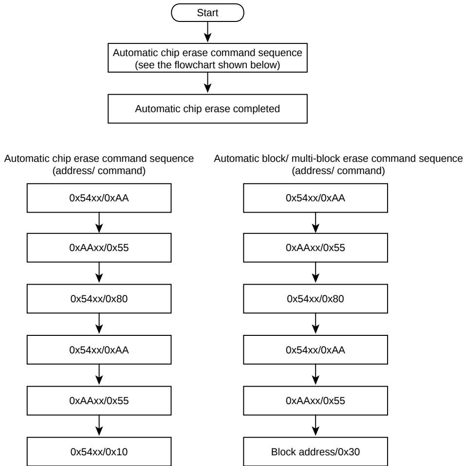
Figure 17-13 Automatic Erase
