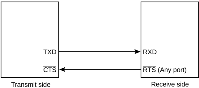
Figure 10-7 Handshake Function
