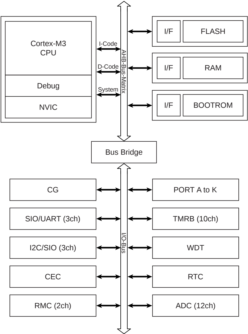
Figure 1-1 TMPM330FDFG/FYFG/FWFGBlock Diagram
