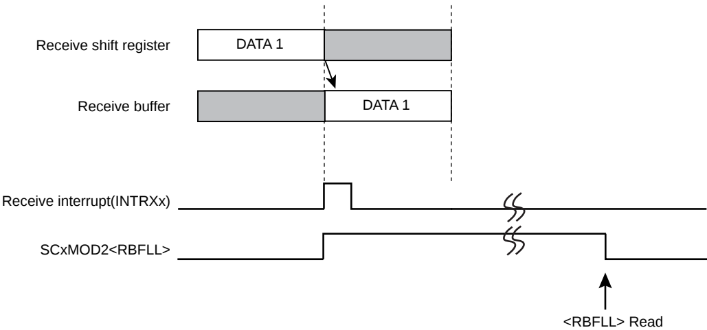
Figure 10-3 Receive Buffer Operation
