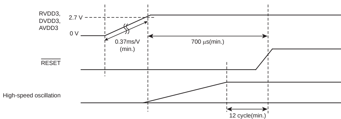
Figure 19-2 Power-on sequence
