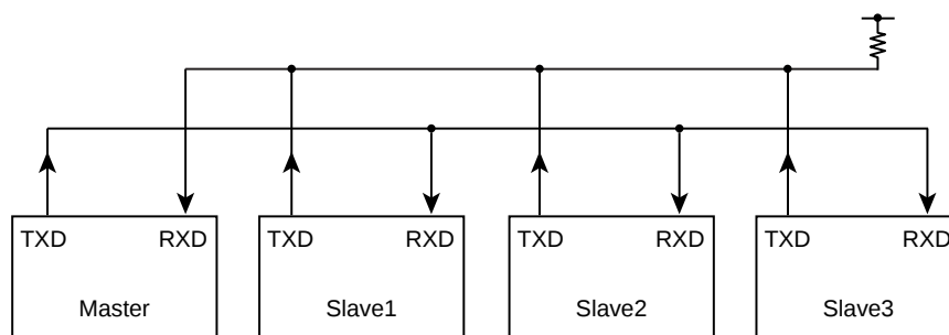
Figure 10-15 Serial Links to Use Wake-up Function
