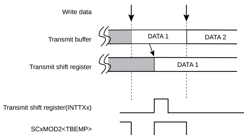
Figure 10-6 Operation of Transmission Buffer
