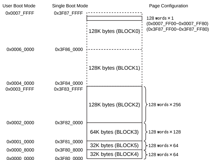
Figure 17-10 Block Configuration of Flash Memory (TMPM330FYFG)
