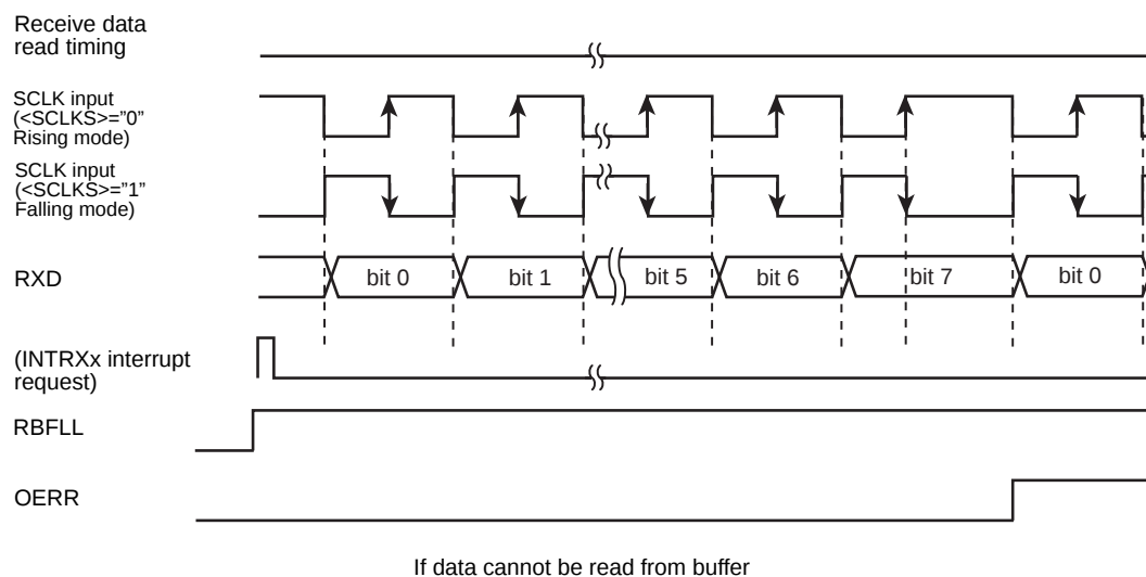
Figure 10-12 Receive Operation in the I/O Interface Mode (SCLK Input Mode)
