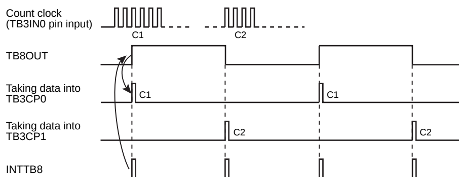
Figure 9-7 Frequency Measurement
