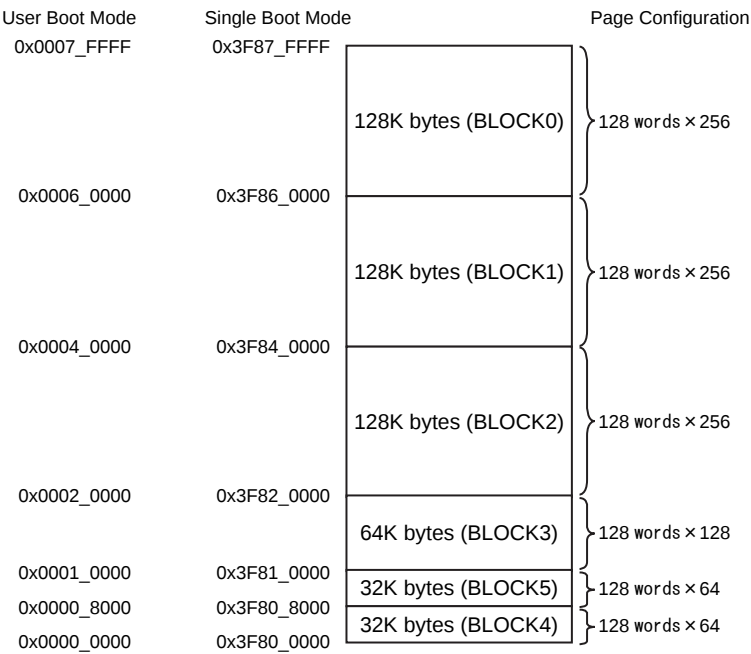
Figure 17-9 Block Configuration of Flash Memory (TMPM330FDFG)
