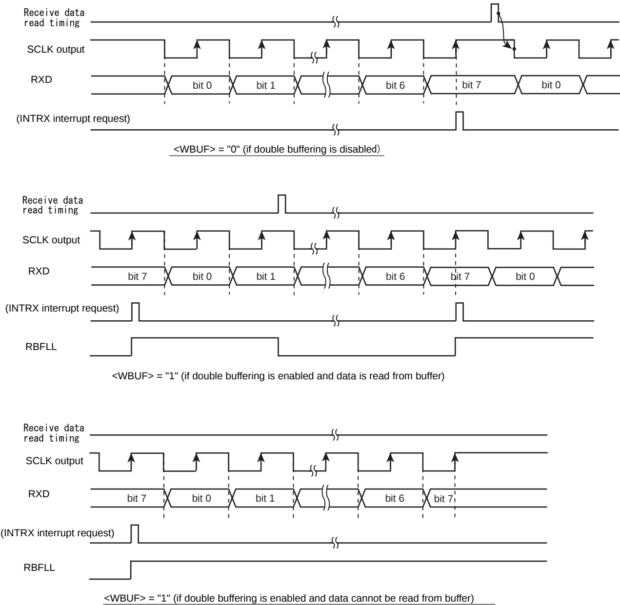
Figure 10-11 Receive Operation in the I/O Interface Mode (SCLK Output Mode)
