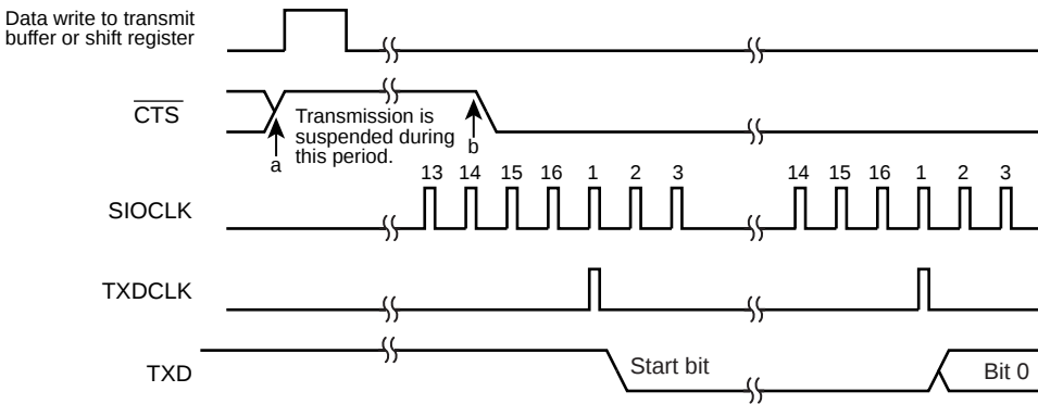
Figure 10-8 \overline{\text{CTS}} Signal timing
