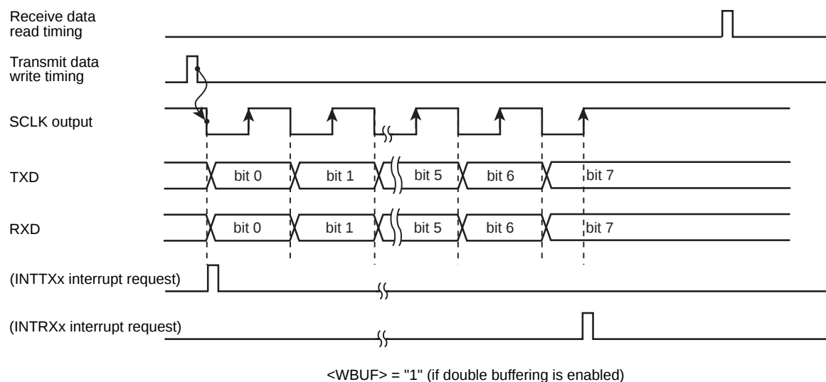
Figure 10-13 Transmit/Receive Operation in the I/O Interface Mode (SCLK Output Mode)
