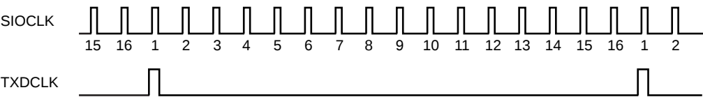
Figure 10-5 Generation of Transmission Clock
