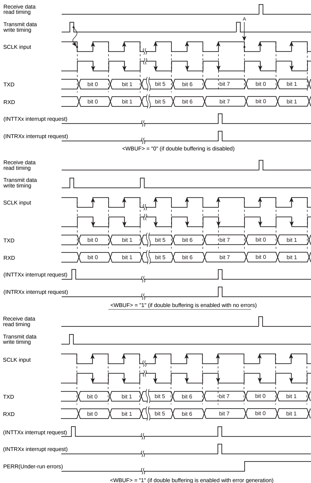
Figure 10-14 Transmit/Receive Operation in the I/O Interface Mode (SCLK Input Mode)
