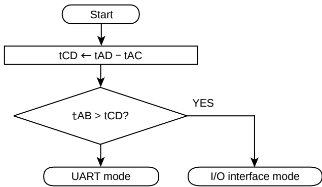
Figure 17-6 Serial Operation Mode Determination Flowchart
