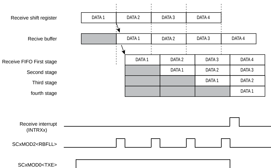
Figure 10-4 Receive FIFO Operation
