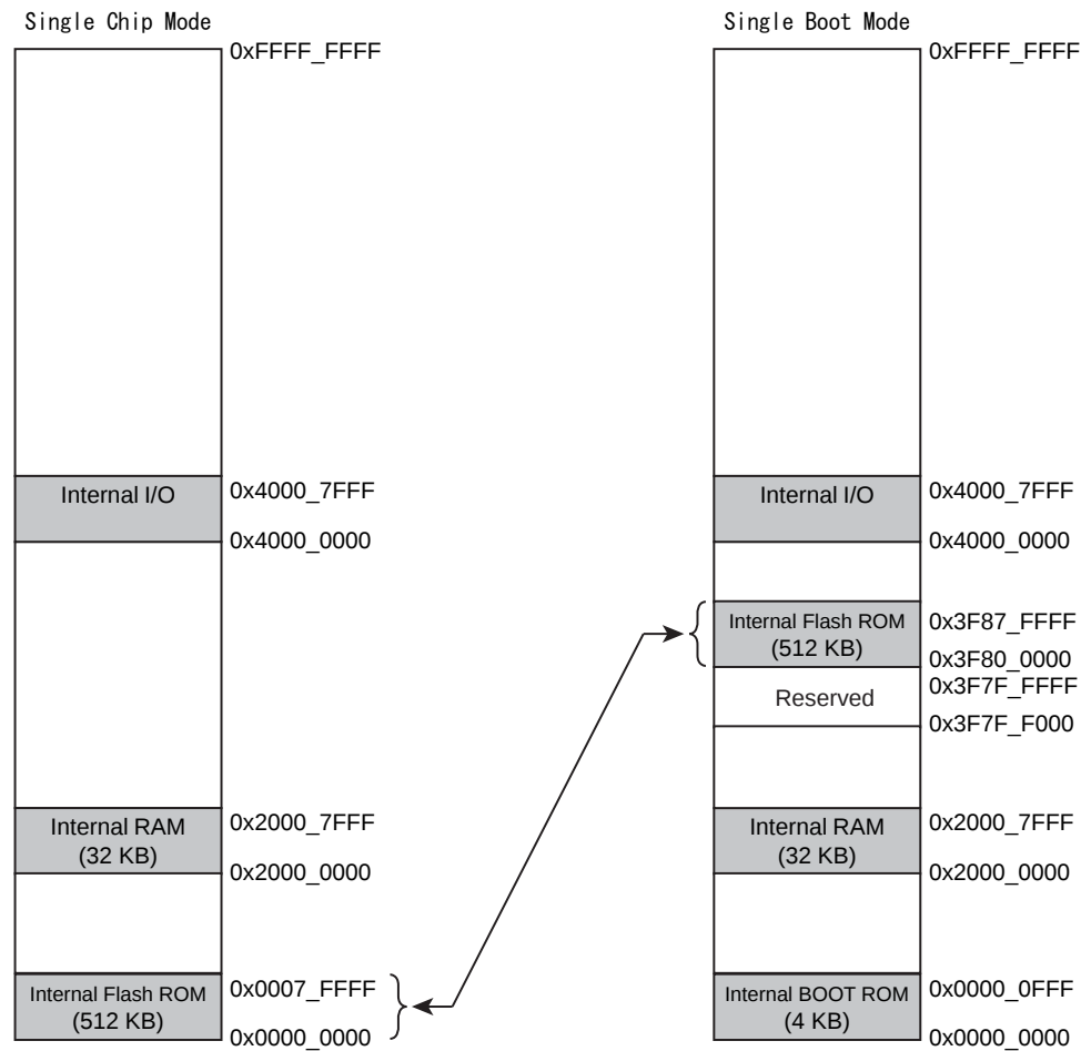
Figure 17-3 Memory Maps for TMPM330FD
