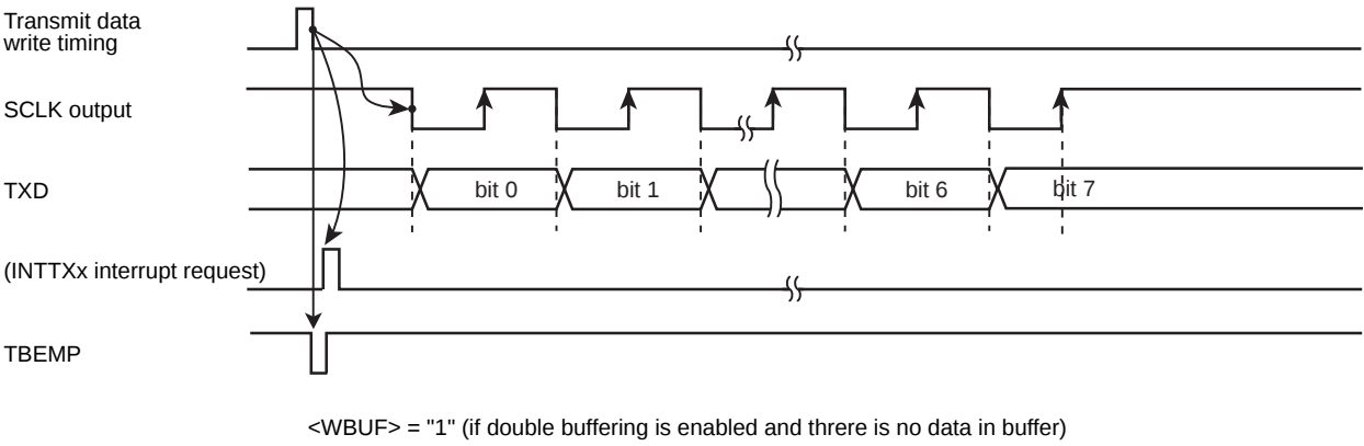
Figure 10-9 Transmit Operation in the I/O Interface Mode (SCLK Output Mode)
