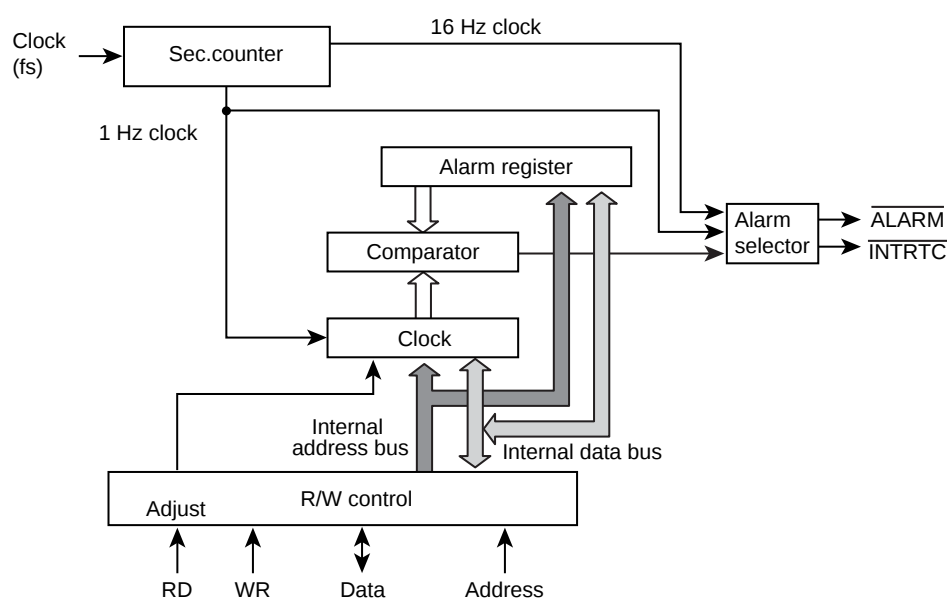
Figure 16-1 Block Diagram
