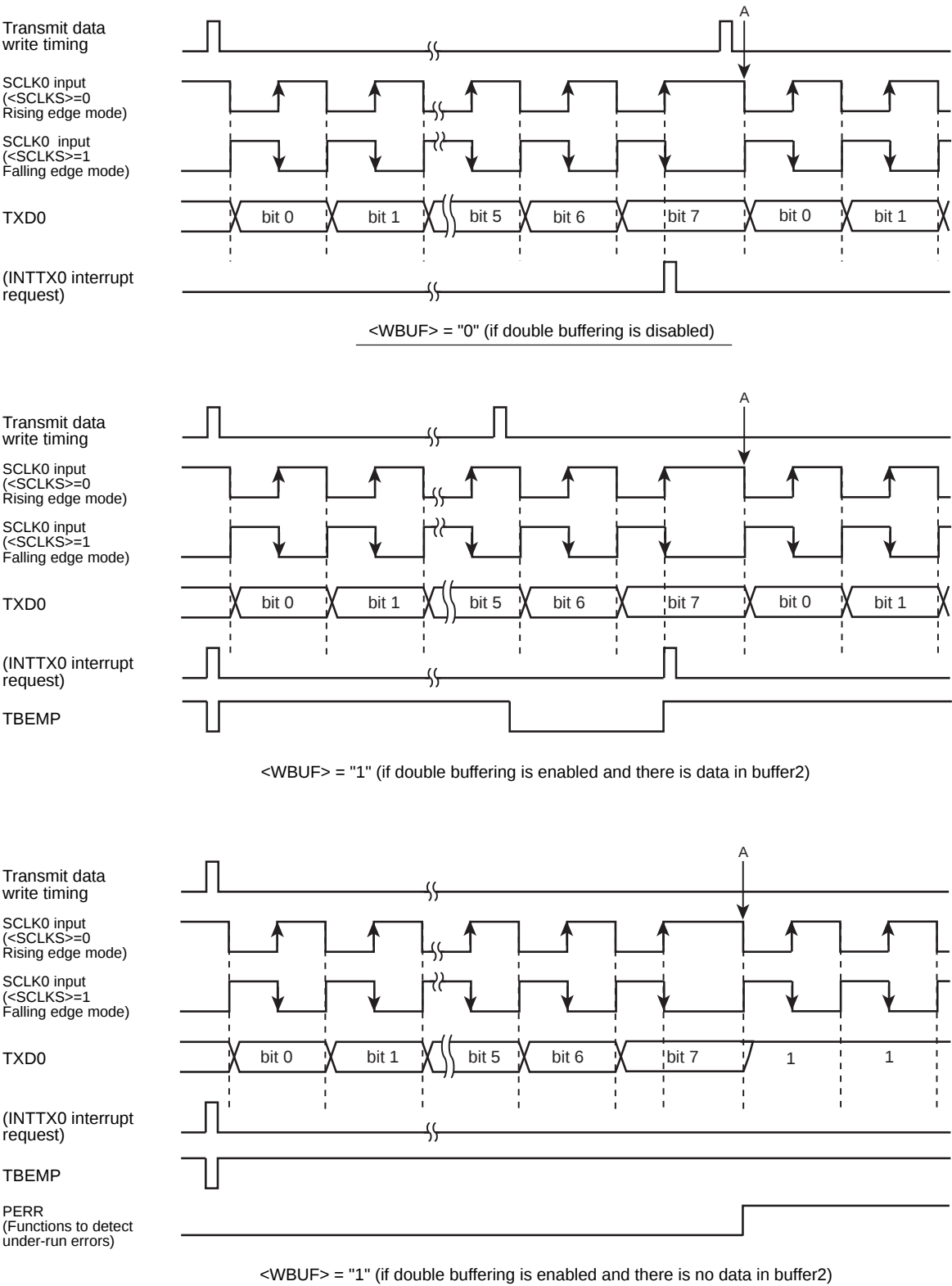
Figure 10-10 Transmit Operation in the I/O Interface Mode (SCLK Input Mode)
