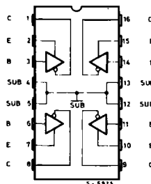
ULN2074B ULN2076B
