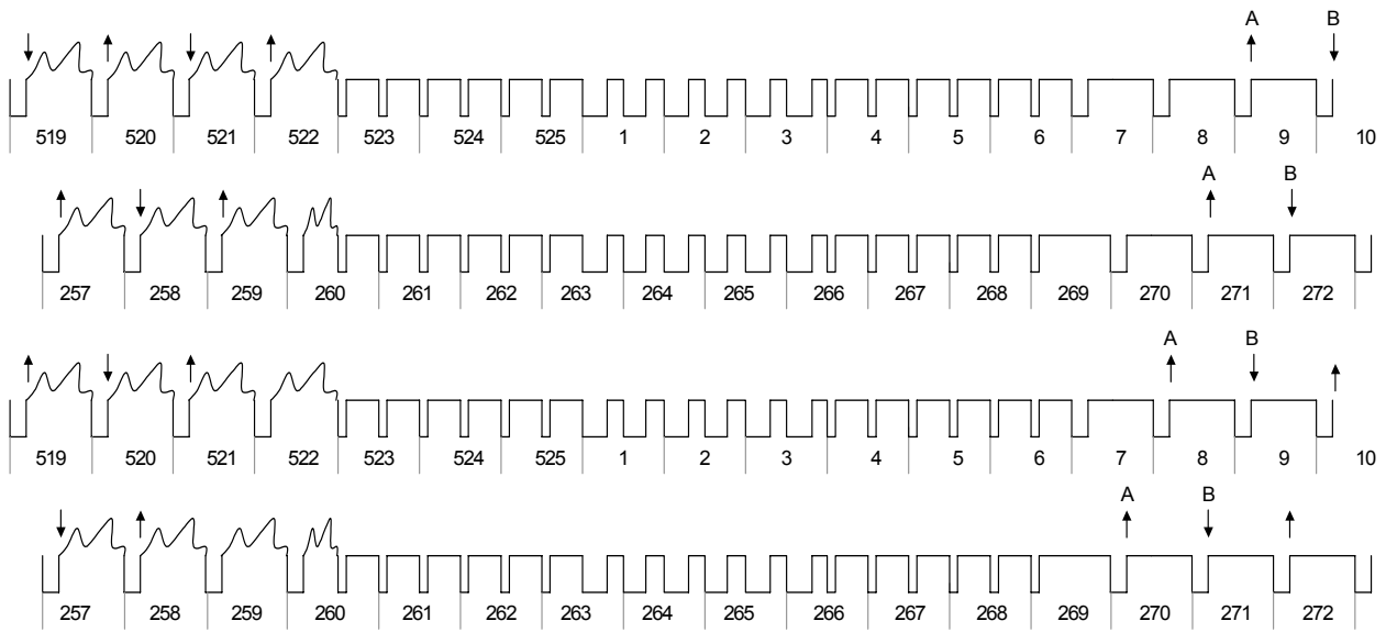
Fig. 19 FID/VSNC Timing and Phase of Burst
