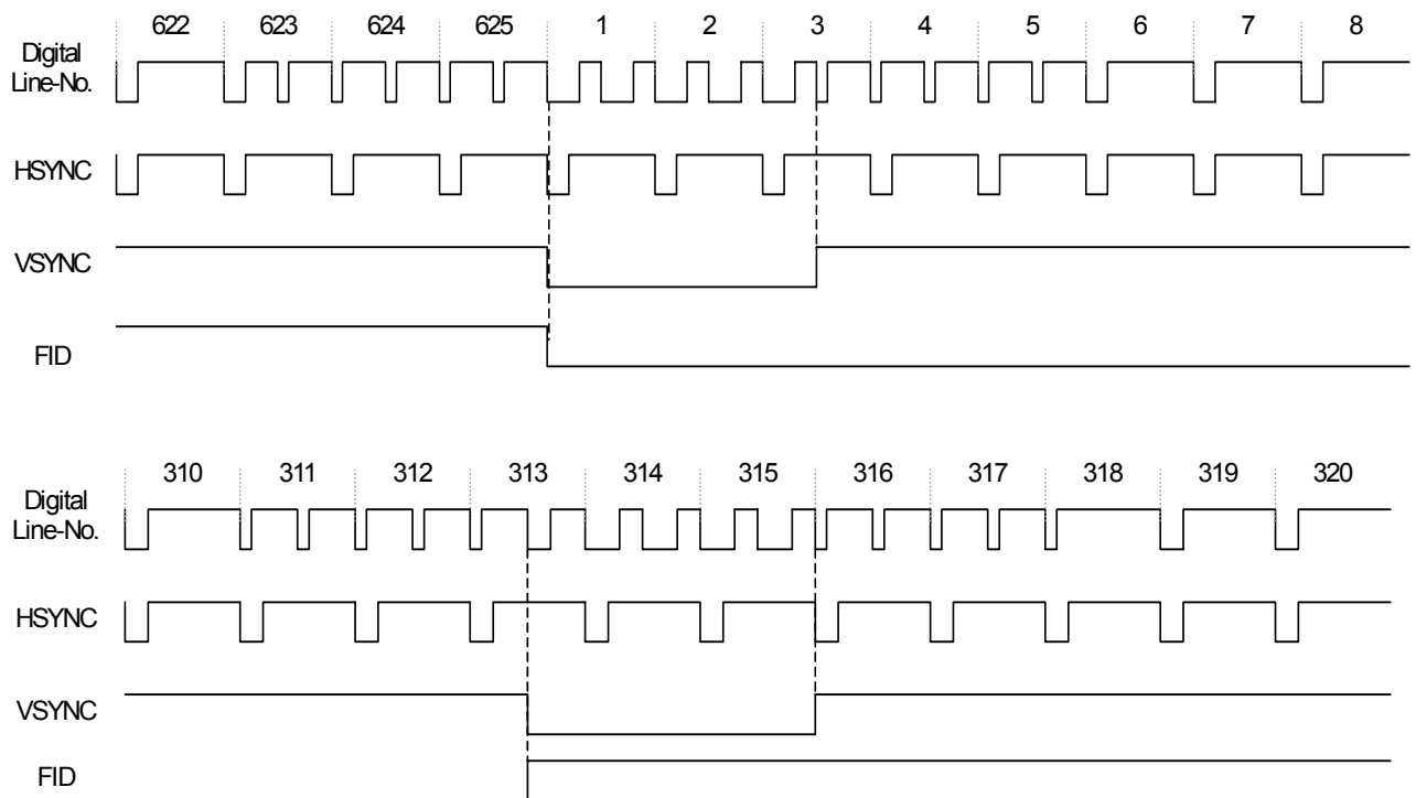
Fig. 13 HSYNC FID/VSNC Timing
