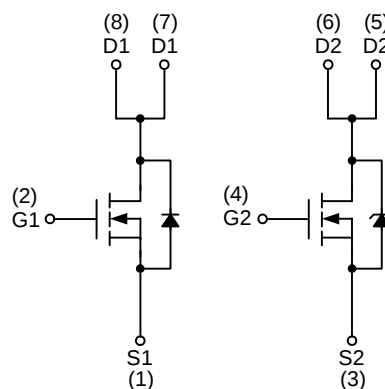
N-Channel MOSFET
