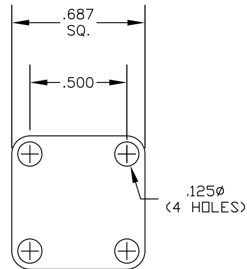
MOUNTING HOLES
