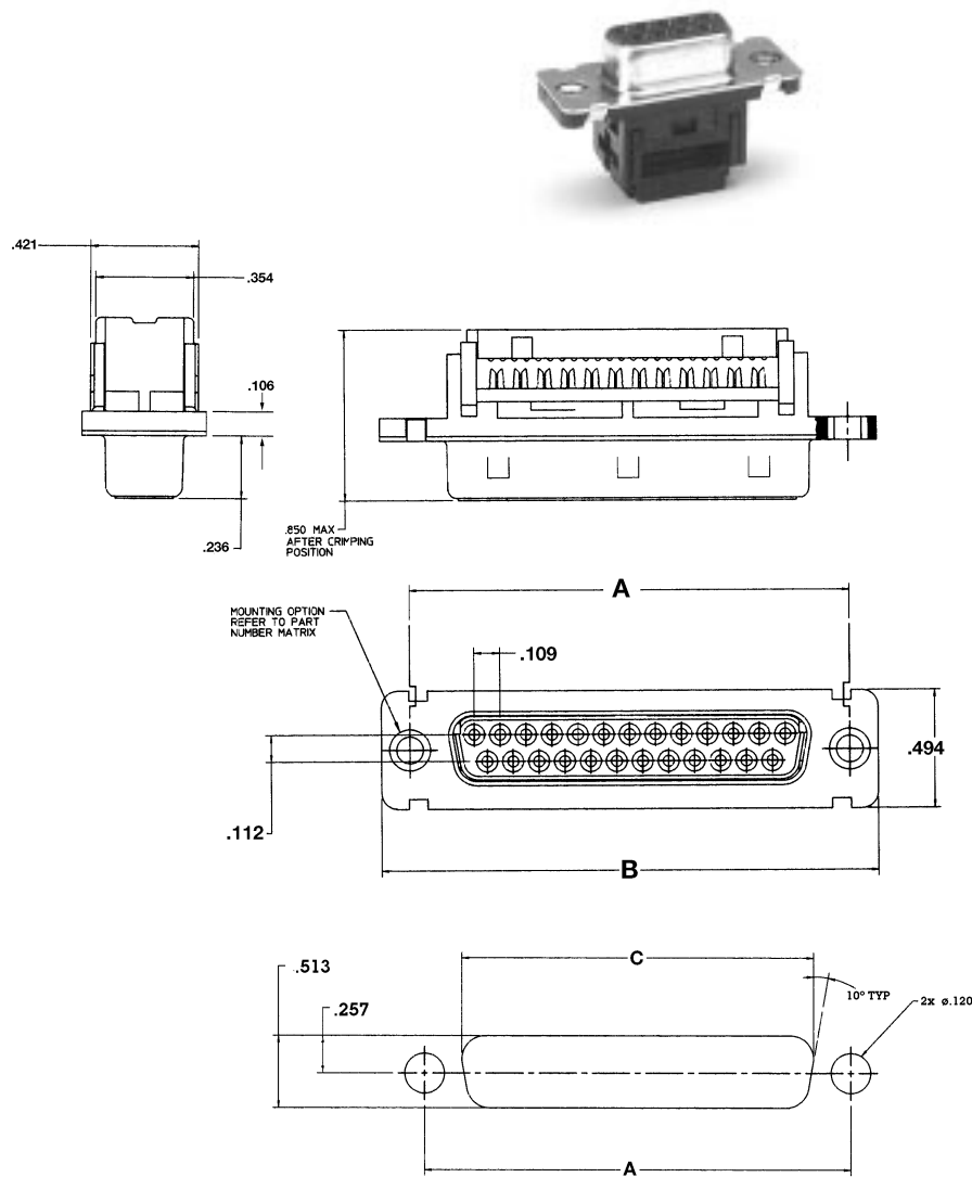
RECOMMENDED PANEL CUTOUT DIMENSIONS
