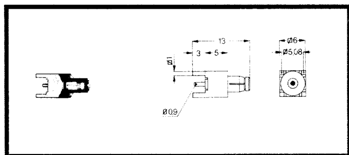
FPA Straight Plug, Non-Latching, for Printed Circuit
