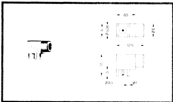
EPL Elbow Receptacle (90°) for Printed Circuit
