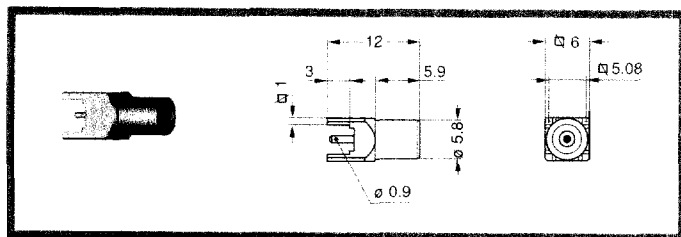
EPA Fixed Receptacle for Printed Circuit
