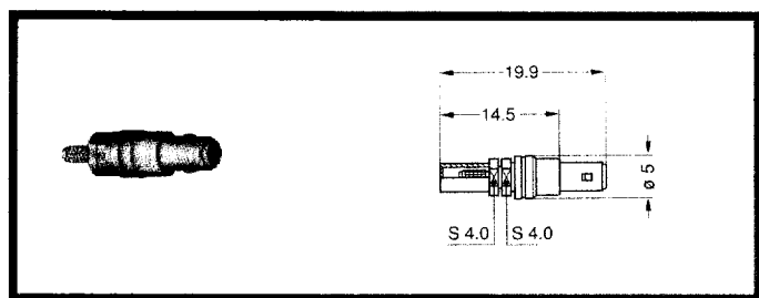
FFS Straight Plug for Cable Crimping
