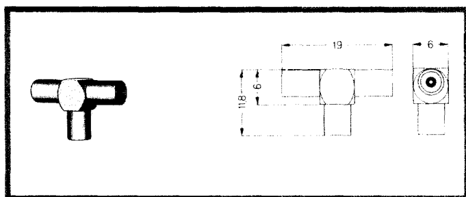
RTA T-coupler with Three Receptacles
