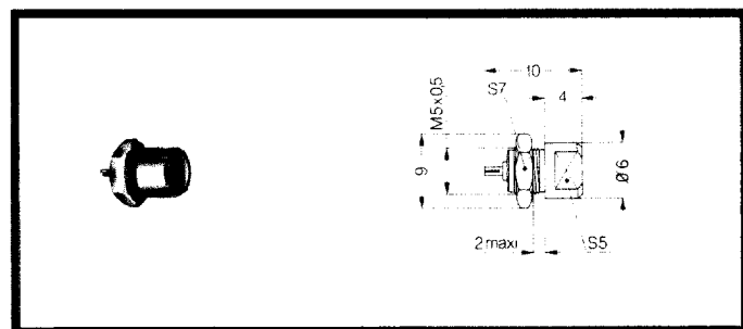
ERA Fixed Receptacle, Nut Fixing
