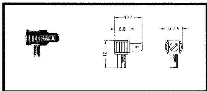
FLS/FLH (Non-Latching) Elbow Plug (90°) for Cable Crimping
