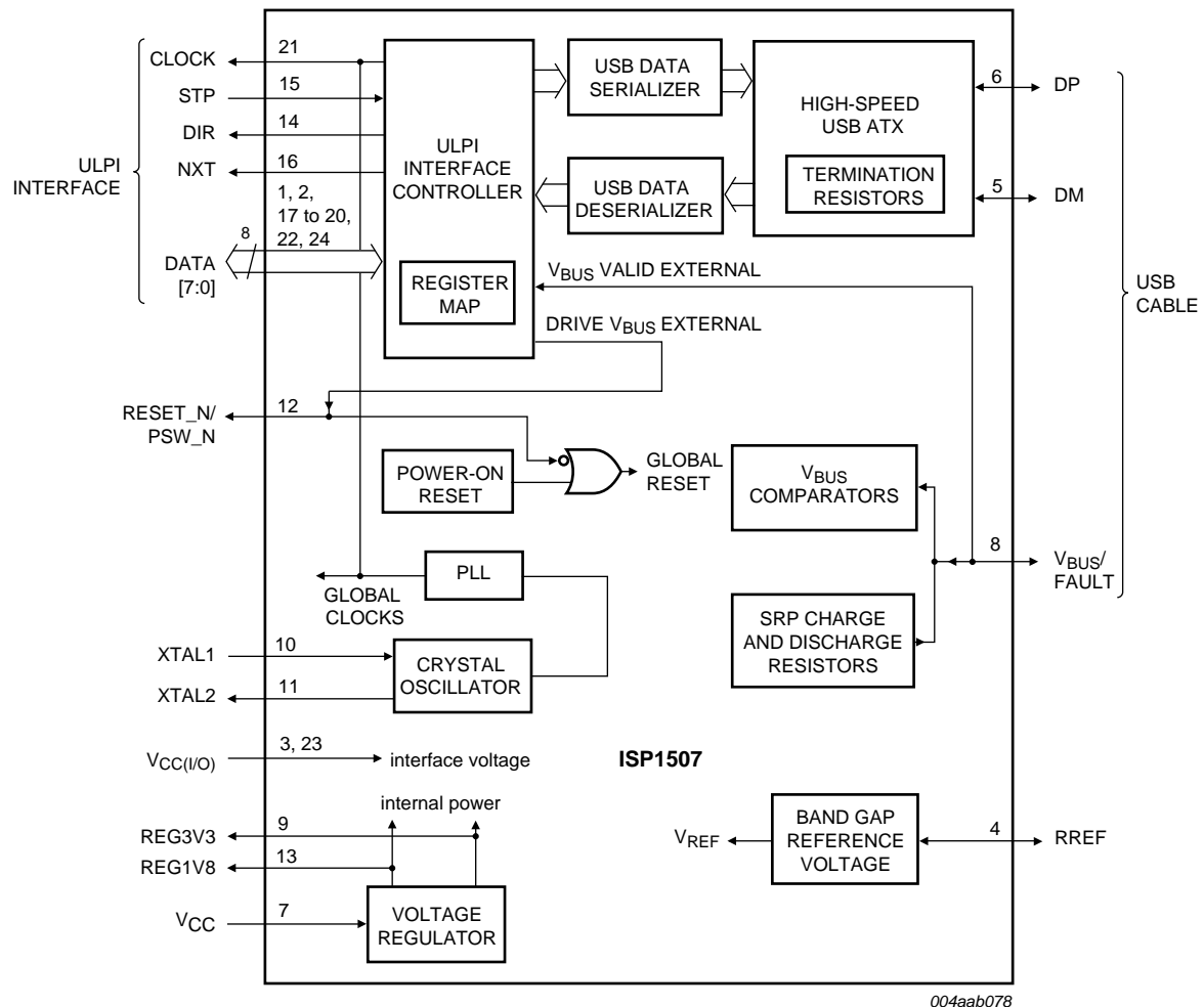
Fig 1. Block diagram
