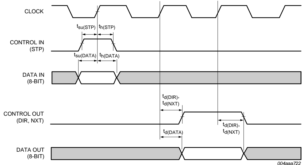
Fig 25. ULPI timing
