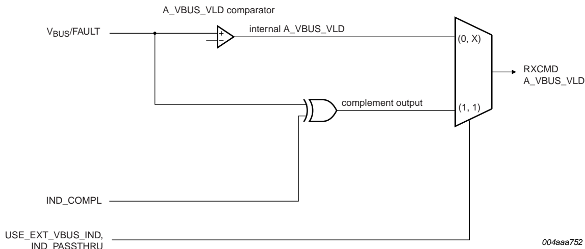
Fig 7. RXCMD A_VBUS_VLD indicator source
