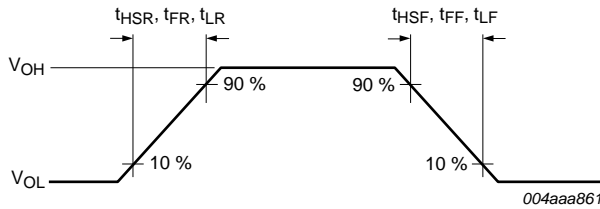
Fig 21. Rise time and fall time
