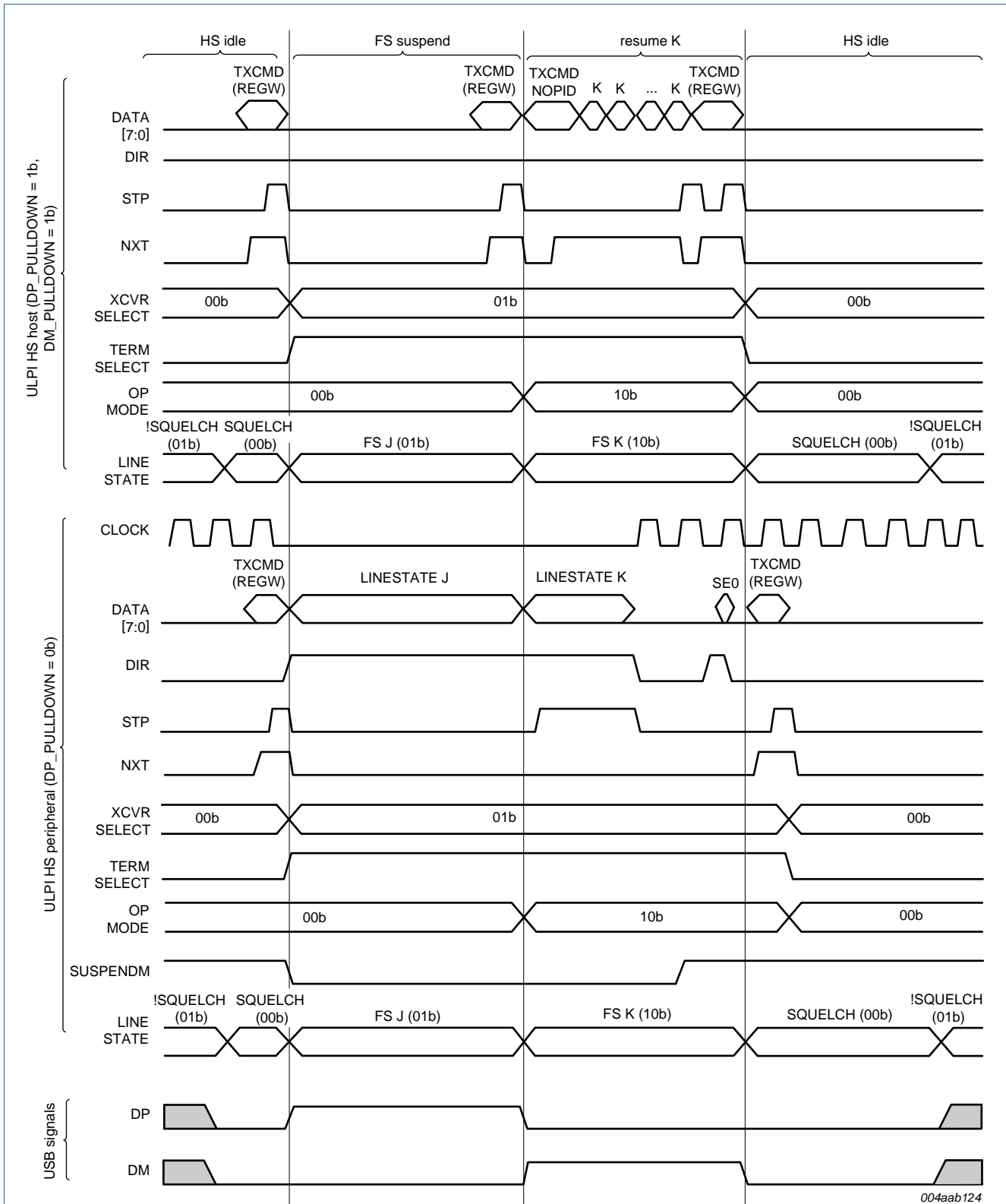
Fig 15. High-speed suspend and resume
