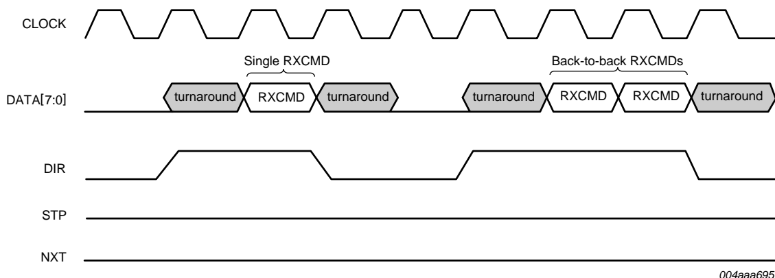
Fig 6. Single and back-to-back RXCMDs from the ISP1507 to the link
