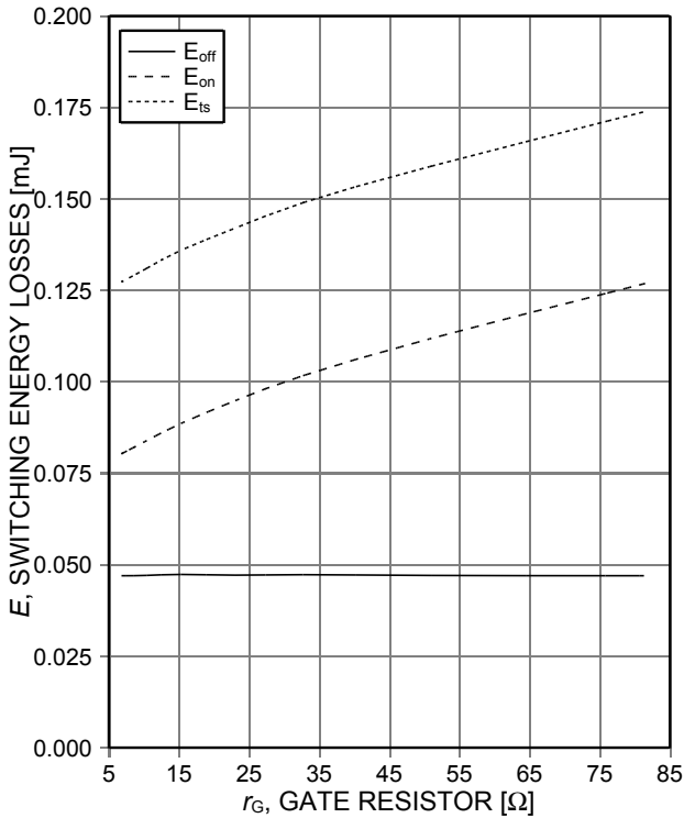
Figure 13. Typical switching energy losses as a function of gate resistor (inductive load, T_{vj}=150^{\circ}C , V_{CE}=400V , V_{GE}=15/0V , I_C=4A , Dynamic test circuit in Figure E)
