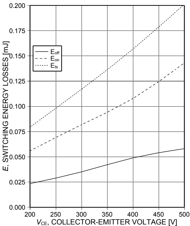
Figure 15. Typical switching energy losses as a function of collector emitter voltage (inductive load, T_{vj}=150^{\circ}C , V_{GE}=15/0V , I_C=4A , r_G=48\Omega , Dynamic test circuit in Figure E)
