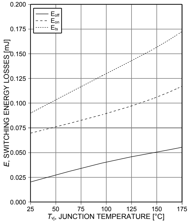
Figure 14. Typical switching energy losses as a function of junction temperature (inductive load, V_{CE}=400V , V_{GE}=15/0V , I_C=4A , r_G=48\Omega , Dynamic test circuit in Figure E)
