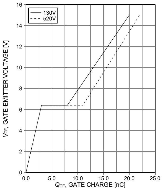
Figure 16. Typical gate charge ( I_C=8A )
