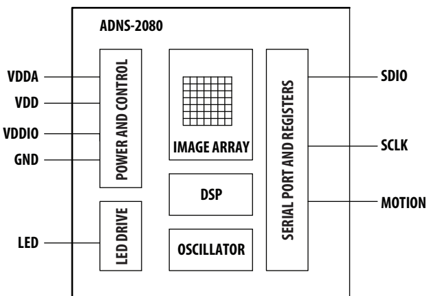
Figure 7. Block diagram of ADNS-2080 optical mouse
