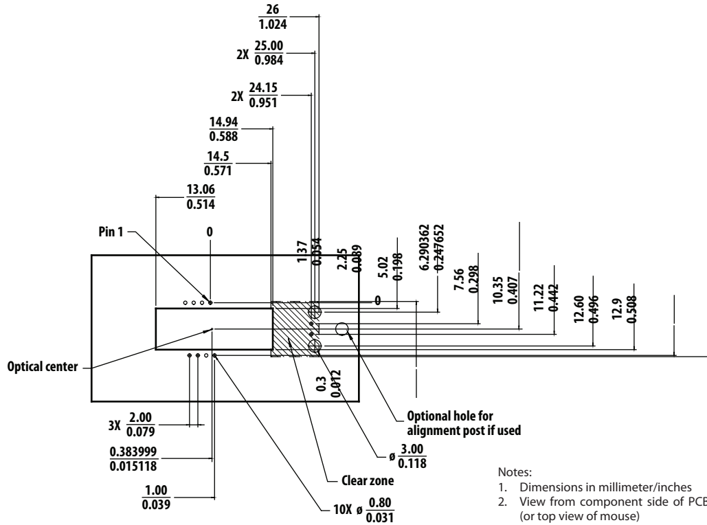
Figure 3. Recommended PCB Mechanical Cutouts and Spacing
