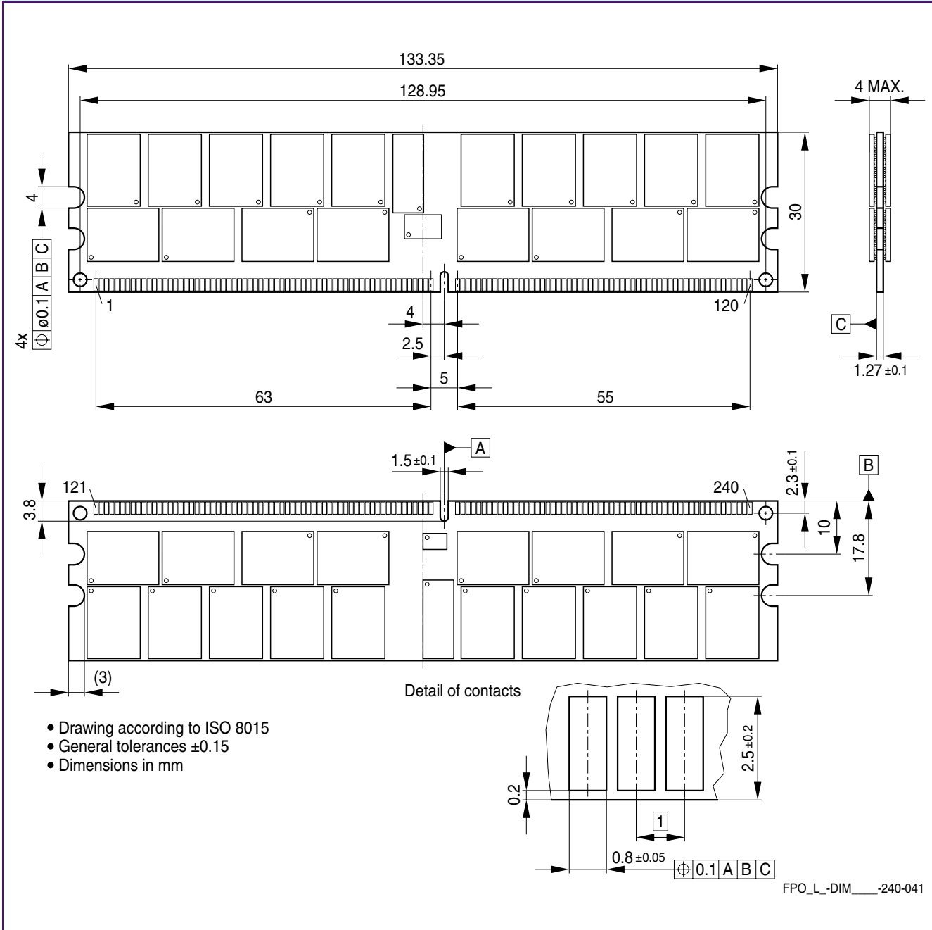
FIGURE 8 Package Outline L-DIM-240-41 Raw Card Z
