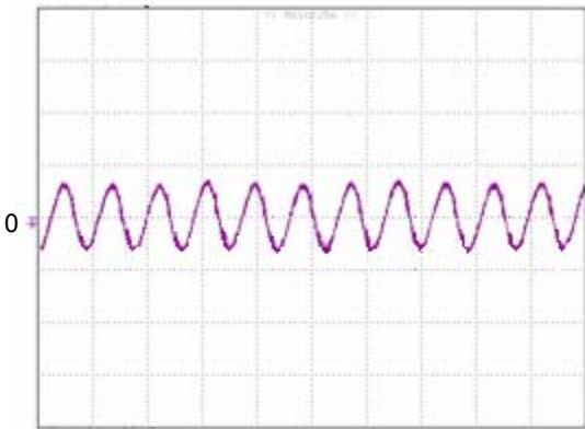
Figure 10: Input reflected ripple current, i_s , through a 12\mu H source inductor at nominal input voltage ( V_{in}=48V ) and rated load current ( 20\text{ mA/div} , 5\mu s/div )
