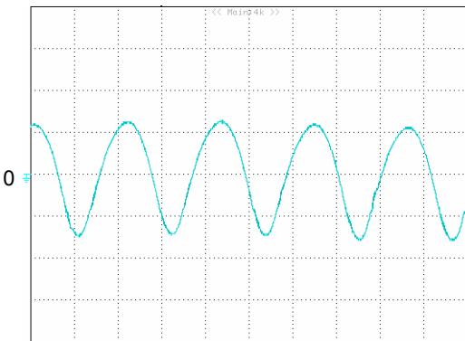
Figure 12: Output voltage ripple at nominal input voltage ( V_{in}=48V ) and rated load current ( 50\text{ mV/div} , 2\mu s/div ). Load capacitance: 1\mu F ceramic capacitor and 10\mu F tantalum capacitor. Bandwidth: 20\text{ MHz} . Scope measurements should be made using a BNC cable (length shorter than 20 inches). Position the load between 51 mm to 76 mm (2 inches to 3 inches) from the module
