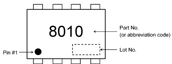
Fig. 7.1 Marking
