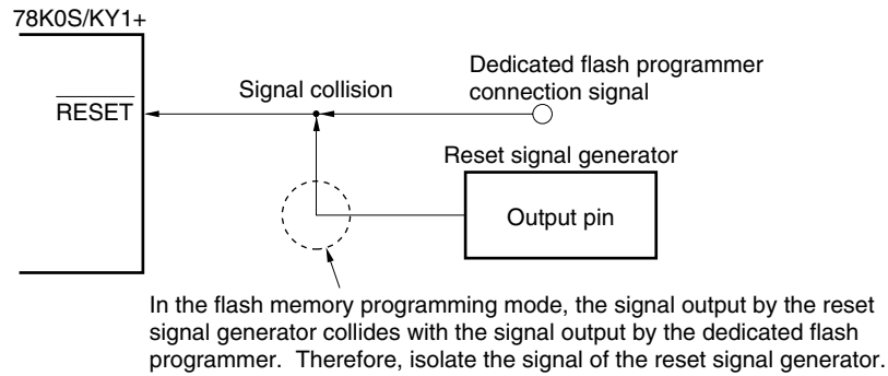
Figure 16-8. Signal Collision ( \overline{\text{RESET}} Pin)
