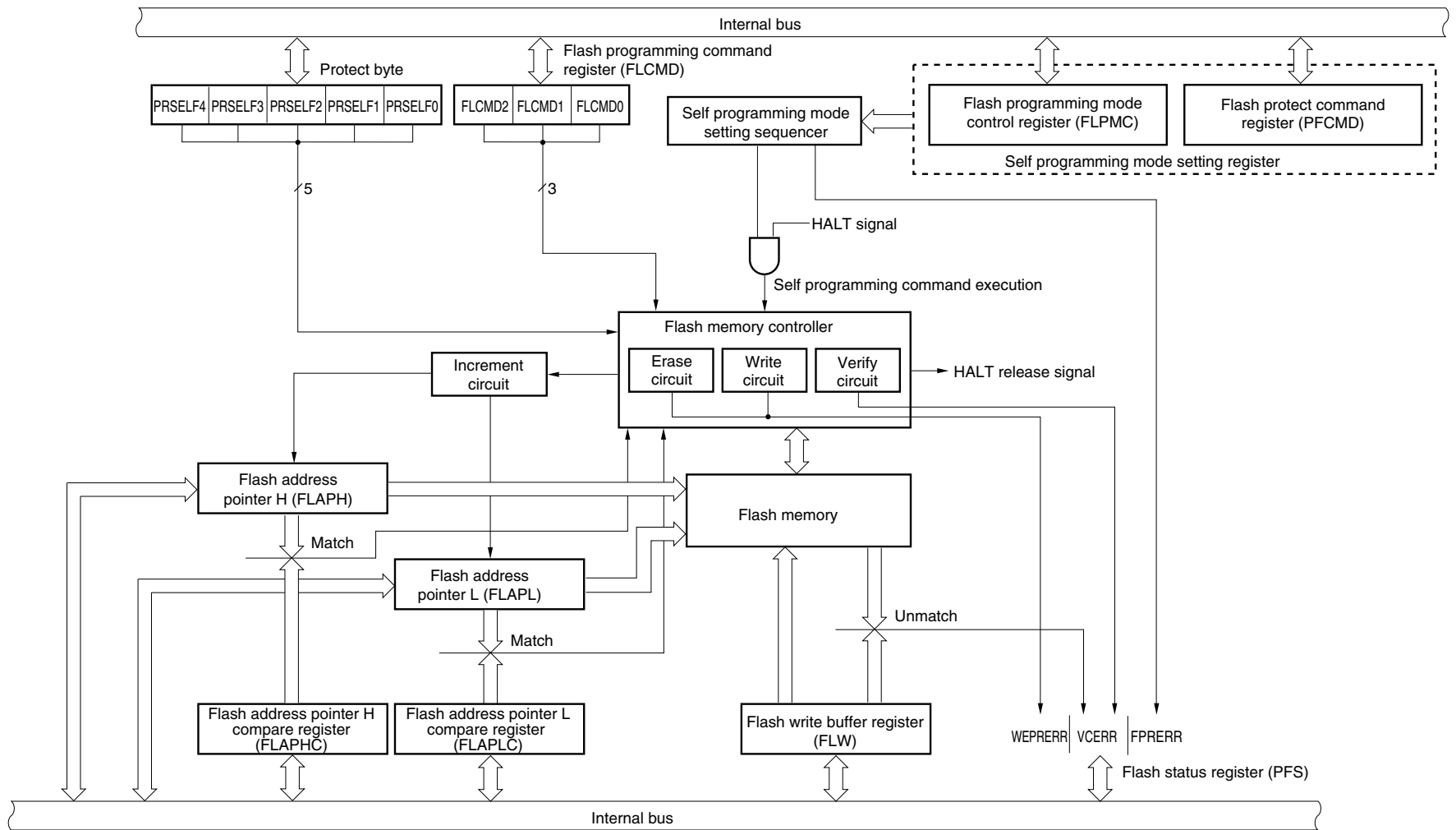
Figure 16-10. Block Diagram of Self Programming
