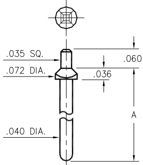
8XXX-X-05-XX-00-00-03-0 Square press-fit in .043 plated thru hole
