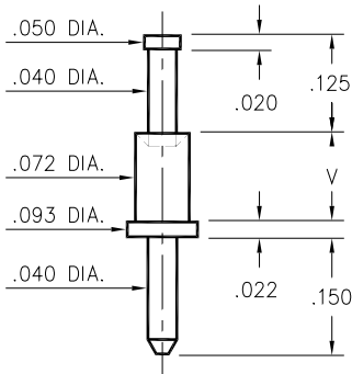
3156-X-00-XX-00-00-08-0 Swage mount in .076 hole
