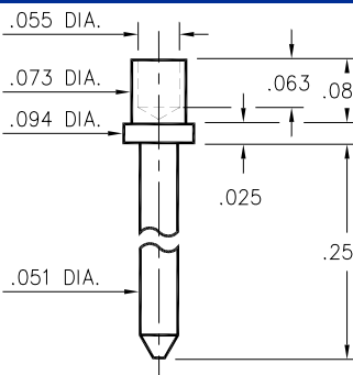
3146-2-00-XX-00-00-08-0 Swage mount in .076 hole. For .062 thick board
