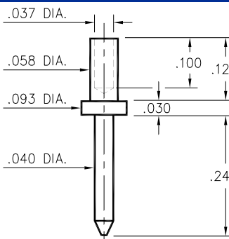
3232-3-00-XX-00-00-08-0 Swage mount in .062 hole. For .094 thick board
