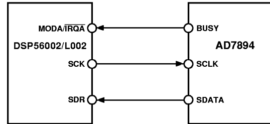
Figure 9. AD7894 to DSP56002/L002 Interface
