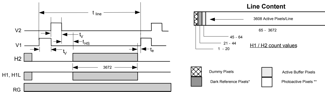
Figure 13: Line Timing
