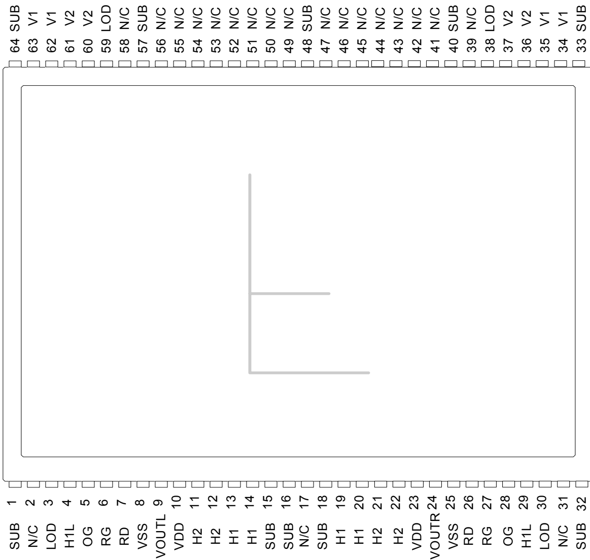
Figure 4: Pinout Diagram
