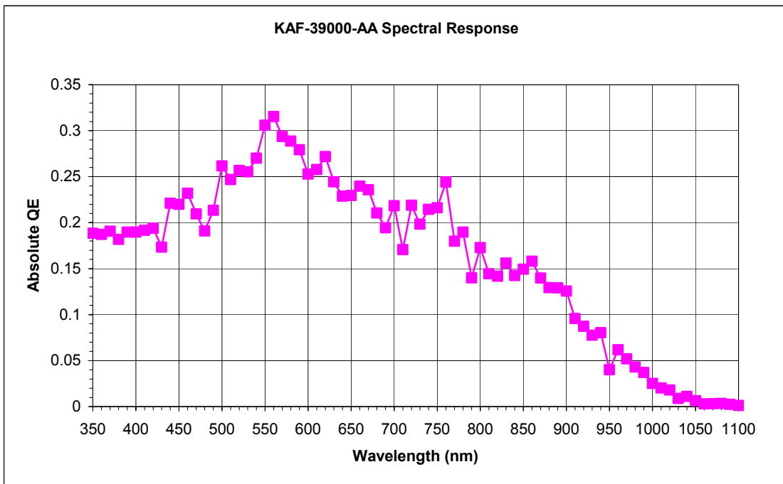
Figure 6: Spectral Response (monochrome version)
