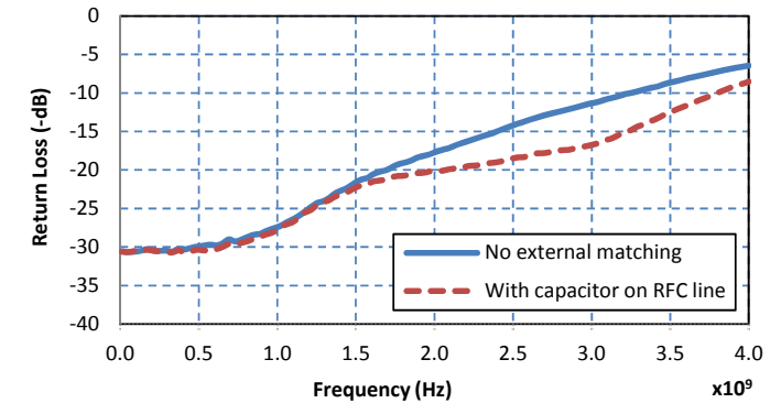
Figure 23. Active Port Return Loss (RF2 Active) 1
