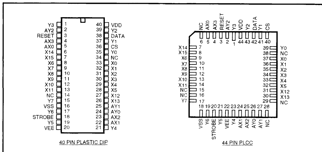
Figure 2 - Pin Connections
