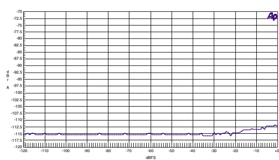
Figure 6. THD + N (dB) vs. Amplitude
