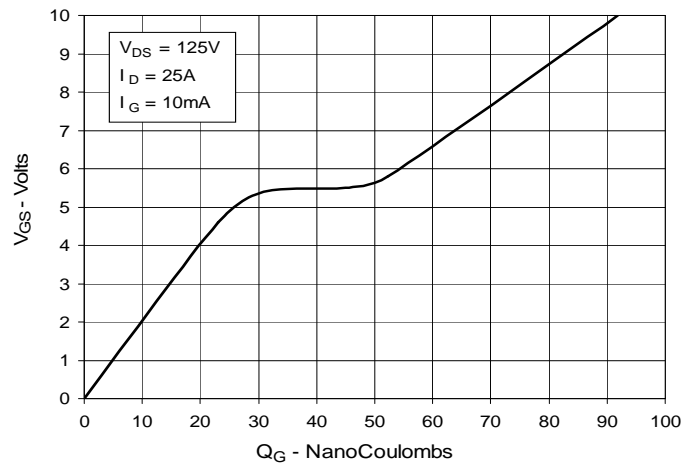
Fig. 10. Gate Charge
