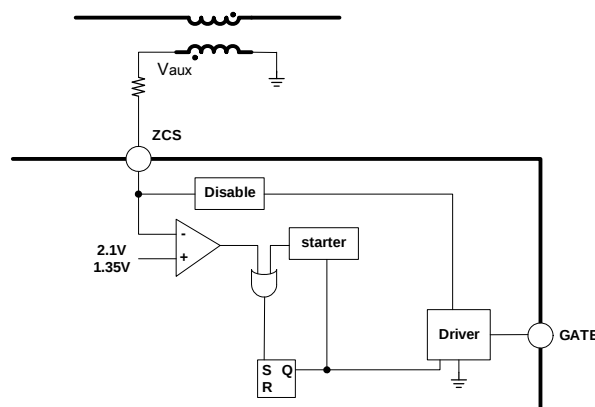
Figure 3: ZCS, Triggering, and Disable Block
