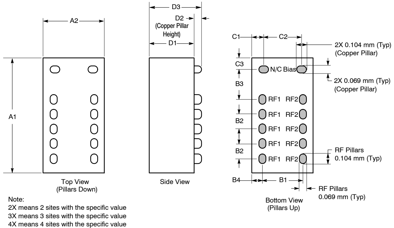
Figure 7. WLCSP Package Dimensions
